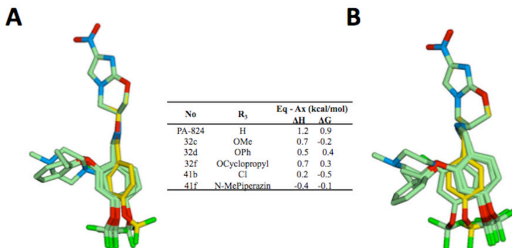
Figure 2. Superpositions of PA-824 ( 1 ) and some R 3 derivatives that were geometry optimized at the level of B3LYP/61-31G*. In each the head, tail and linker region of 1 is shown with yellow carbons, A the tail is shown in the pseudo-equatorial conformation while in B the tail is shown in the pseudo-axial conformation. A and B show R 3 analogs 32c , 32d , 32f , 41b , and 41f . The inset table shows the difference in enthalpy (ΔH) and Gibbs free energy (ΔG) at 298.15 K calculated for the pseudo-equatorial conformer compared with the pseudo-axial conformer for each compound with a solvent reaction field of cyclohexane. Atoms represented by colors are as follows: green, carbon; dark green, fluorine or chlorine; blue, nitrogen; red, oxygen. Hydrogen atoms are not shown.
