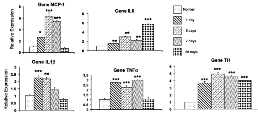
Figure 2. Time course of chronic hypoxia (CH)-induced inflammatory cytokine, and tyrosine hydroxylase (TH) gene expression in rat carotid body. Quantitative PCR data normalized to 18sRNA and expressed relative to mRNA levels in normal tissue. MCP-1: monocyte chemoattractant protein-1; IL6: interleukin-6; IL 1b: interleukin-1β; TNFα: tumor necrosis factor-α. *, **, and *** indicate p<0.05, 0.01 and 0.001, respectively. CH: exposure at 380 Torr for time indicated. (From Liu, He et al. 2009)
