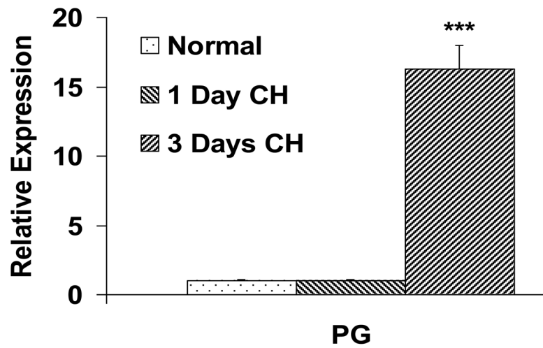
Figure 7. Time course of chronic hypoxia (CH)-induced up-regulation of NaV1.7 \alpha -subunit of voltage gated Na + -channel. Quantitative PCR data normalized to 18sRNA and expressed relative to mRNA levels in normal tissue.
