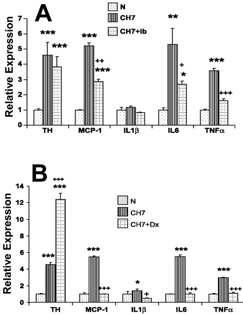
Figure 4. Effect of ibuprofen, A, (ib; 4 mg/kg/day) or dexamethasone, B, (DX; 0.1 mg/kg/day) on 7 day CH-induced gene expression of tyrosine hydroxylase and cytokines in rat carotid body. Abbreviations as in figure 2. *, **, and *** indicate p < 0.05 , 0.01 , and 0.001 , respectively, vs. normal; +, ++, and +++, p < 0.05 , 0.01 , and 0.001 , respectively, vs. 7 days CH. (Adapted from Liu, He et al. 2009)
