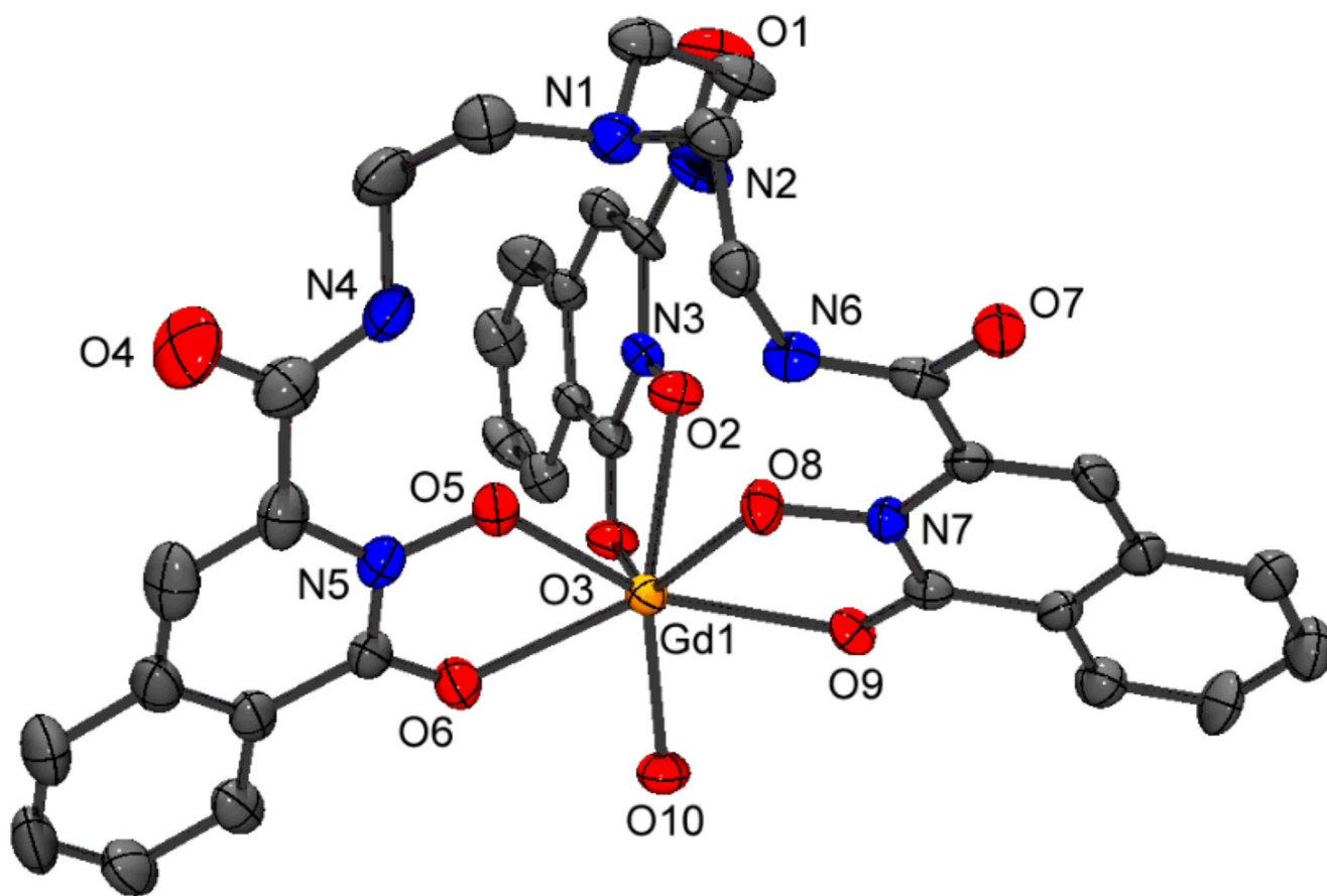
Figure 1. Asymmetric unit of [Gd(1)(H 2 O)] · H 2 O. Thermal ellipsoid plot (ORTEP-3 for Windows, 10 50% probability level) with atom numbering scheme. Hydrogens and the isolated water molecule are omitted for clarity. O7 is coordinated to a neighboring complex.
