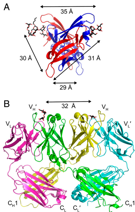
Fig. 5. Similarity in carbohydrate binding site spacing in CV-N and the 2G12 anti-HIV (Fab) 2 . (A) Each of the four carbohydrate binding sites in one WT CV-N crystal structure (15) (P4 1 2 1 2 space group) is approximately 30 to 35 Å from the other sites (structure is viewed from the bottom with respect to Fig. 1). Carbohydrates (shown as sticks with black carbons and red oxygens) were only resolved in the A binding sites in the crystal structure. (B) Ribbon diagram of the domain-swapped (Fab) 2 from IgG 2G12, a broadly neutralizing antibody specific for carbohydrates on gp120 (35). The domain swapping creates a rigid (Fab) 2 dimer in which the carbohydrate binding sites at the antigen combining sites are spaced approximately 30 to 35 Å apart. Carbohydrates are shown as sticks with black carbons and red oxygens and antibody domains are labeled.
