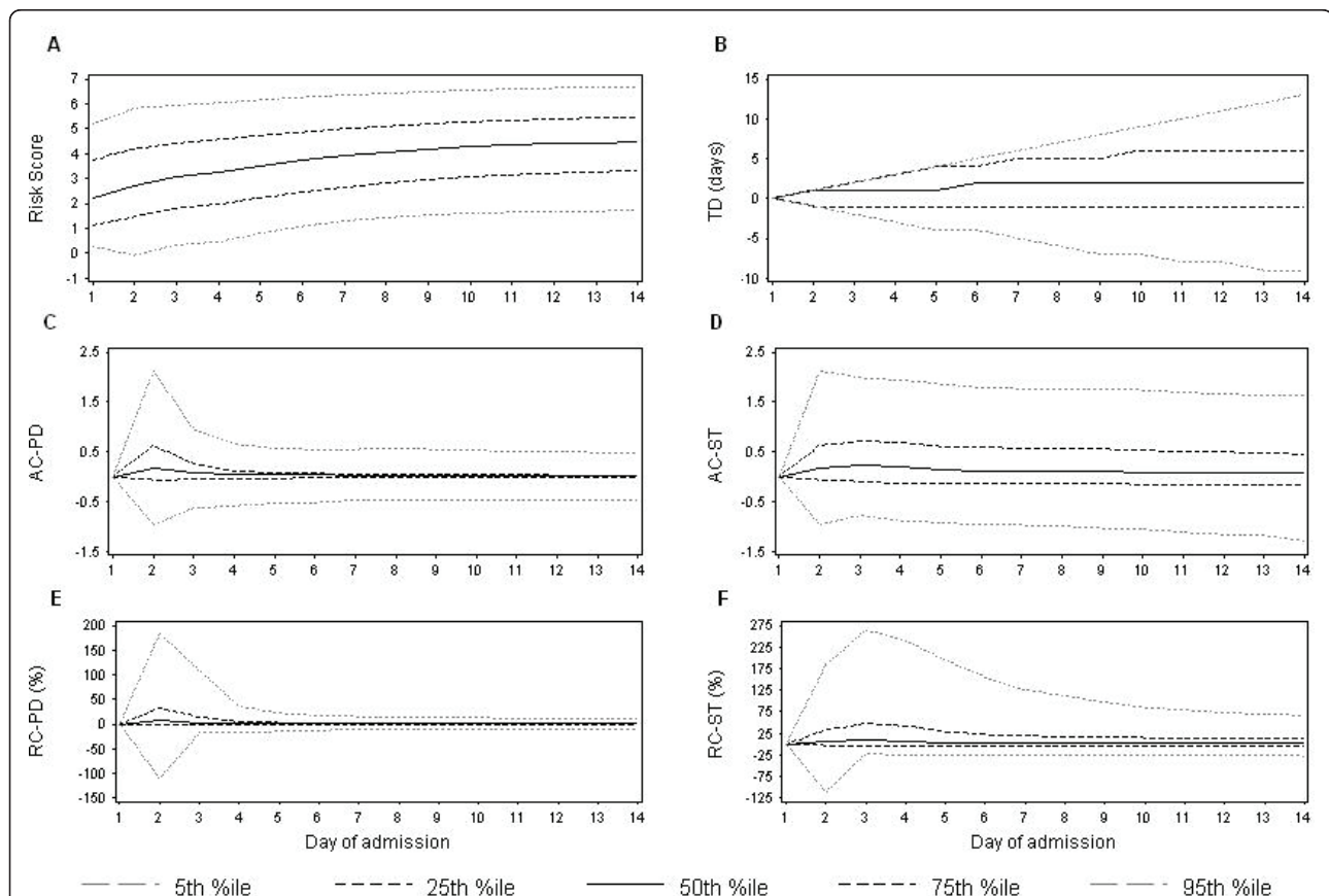
Figure 1 Distribution of the risk score from the existing time-dependent survival model and the trend indicators over time. The graphs above show the value of the risk score from the existing time-dependent survival model (Figure 1A) and the five trend indicators (Figure 1B-1F) at the 5 th , 25 th , 50 th , 75 th , and 95 th percentile of observed values on each of the first 14 days of admission. The value of each trend indicator is positive or negative for an increase or decrease in the risk score, respectively. TD = number of consecutive days with a trend in the risk score; AC-PD = absolute change in the risk score from the previous day; AC-ST = absolute change in the risk score from the start of the trend; RC-PD = relative percent change in the risk score from the previous day; RC-ST = relative percent change in the risk score from the start of the trend.
