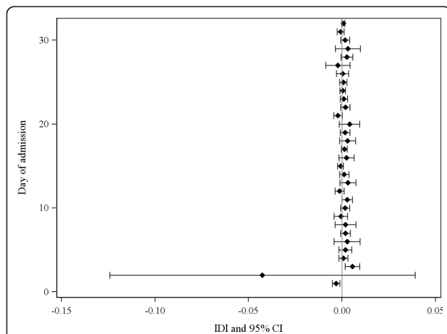
Figure 3 Integrated discrimination improvement (IDI) with 95% confidence intervals (CI) comparing the existing model with and without the trend indicators. On each of the first 32 admission days (the 95 th percentile of observed length of stay), we calculated the IDI with 95% CIs [12] using patients' estimated hazard of death from each model and vital status for that day . An IDI above 0 suggests that the addition of the trend indicators to the existing model improved overall model discrimination.
