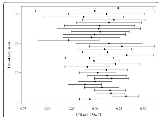
Figure 4 Net reclassification improvement (NRI) with 95% confidence intervals (CIs) comparing the existing model with and without the trend indicators. On each of the first 32 admission days (the 95 th percentile of observed length of stay), we calculated the NRI with 95% CIs [12] using patients' estimated hazard of death from each model and vital status for that day . An NRI above 0 indicates improved risk prediction with the new model containing the trend indicators.
