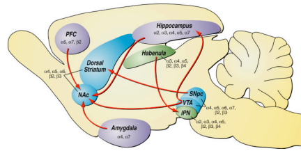
Fig 1. Expression of nAChR subunits in brain regions relevant to nicotine reinforcement Graphical representation of nAChR subtypes expressed in brain regions implicated in the rewarding and reinforcing properties of nicotine and other drugs of abuse. The red arrows indicate neuronal projections. There is dense expression of nAChR subtypes in the ventral tegmental area (VTA) and substantia nigra pars compacta (SNpc) [64, 126, 260–263], which are two major sites of ascending dopamine projections. Sites of dopaminergic input, including the nucleus accumbens (NAc), dorsal striatum, prefrontal cortex (PFC) and hippocampus [129, 260, 264–266] are also enriched in nAChR subtypes. Other brain sites that have dense nAChR expression and that have been implicated in regulating nicotine self-administration behavior include the medial habenula and interpeduncular nucleus (IPN), and amygdala [260, 264, 267].
