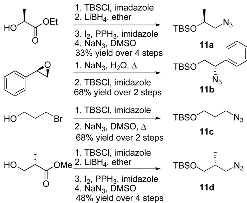
Scheme 3. Silyl ether synthesis
