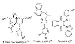
Figure 1. Representative examples of biologically active molecules containing 1,2,3-triazoles.
