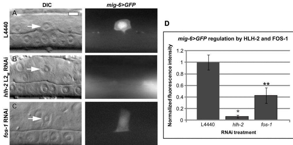
Figure 6. mig-6 is transcriptionally regulated by HLH-2 and FOS-1 in the AC DIC images (left in each lettered pair) and corresponding mig-6>GFP fluorescence images (right in each lettered pair) at the mid-L3 stage. (A) L4440 control RNAi treatment with the AC expressing mig-6>GFP at the P6.p four-cell stage. (B) hlh-2 L2 M RNAi treatment results in undetectable mig-6>GFP expression, and (C) fos-1 RNAi treatment reduces mig-6>GFP expression. (D) Quantification of RNAi treatment. mig-6>GFP expression is reduced 94% by hlh-2 L2 M RNAi treatment and 57% by fos-1 RNAi treatment compared to control conditions. n = 15 ; *p < 1 \times 10^{-8} ; **p < .01 ; error \pm S.E.M.
