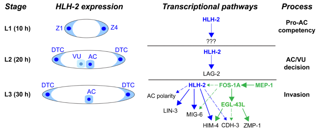
Figure 8. Schematic diagram of HLH-2 expression and activity in the AC through the time of invasion
