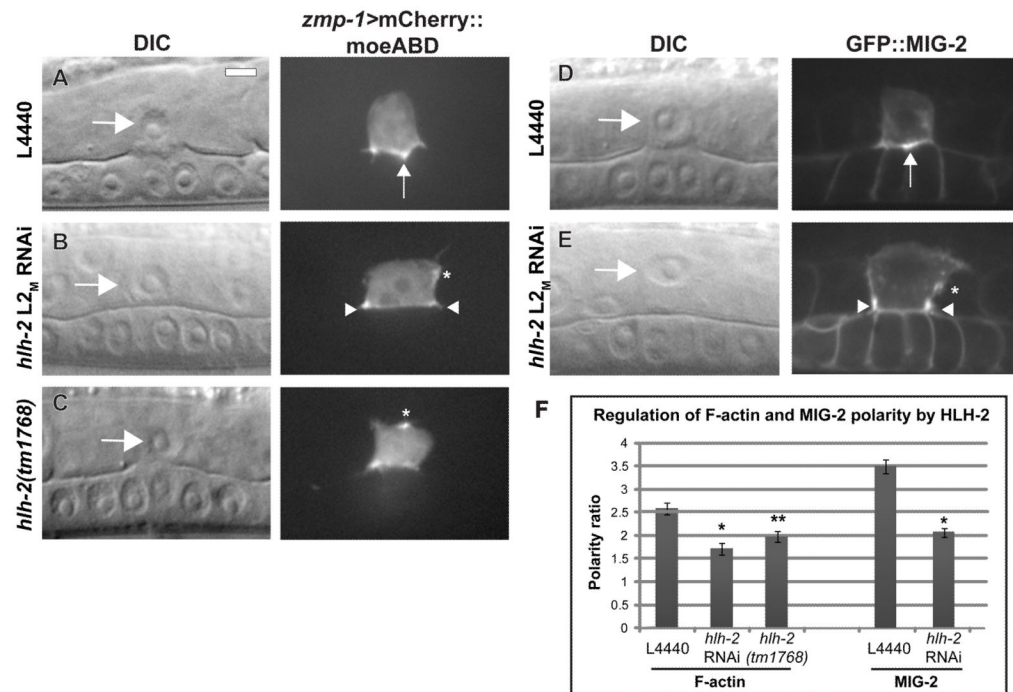
Figure 7. HLH-2 is required for formation of the invasive cell membrane in the AC (A–C) DIC images (left in each lettered pair) and corresponding fluorescence images (right in each lettered pair) at the mid-L3 stage of animals expressing the AC-specific F-actin binding protein zmp-1 >mCherry::moesinABD. (A) In control L4440 RNAi treatment, F-actin localizes to the invasive membrane in contact with the BM and concentrates in the center of the AC between the two central 1° VPCs (arrow). (B) In hlh-2 L2 M RNAi-treated animals, AC invasion is blocked and F-actin localizes on the periphery of the ventral surface, away from the central 1° VPCs (arrowheads). An ectopic patch is mispolarized on the lateral side (asterisk). (C) Despite normal AC invasion in an hlh-2 (tm1768) animal, an apical patch of F-actin is present on the AC plasma membrane (asterisk). (D–E) DIC images (left) and corresponding fluorescence images (right) in the mid-L3 stage of animals expressing the Rac GTPase GFP::MIG-2. (D) In control L4440 RNAi, GFP::MIG-2 concentrates on the ventral surface between the two central 1° VPCs (arrowhead). (E) In hlh-2 L2 M RNAi-treated animals, GFP::MIG-2 localizes on the periphery (arrowheads), and an ectopic patch is present on the lateral side (asterisk). (F) Quantification of F-actin and MIG-2 polarity in control (L4440) and hlh-2 reduction-of-function conditions. Polarity ratio reflects the amount of mCherry::moesinABD or GFP::MIG-2 at the ventral invasive cell membrane relative to the apical and lateral surfaces. n = 15 ; * p < 1 \times 10^{-8} ; ** p < 1 \times 10^{-3} ; error \pm S.E.M.
