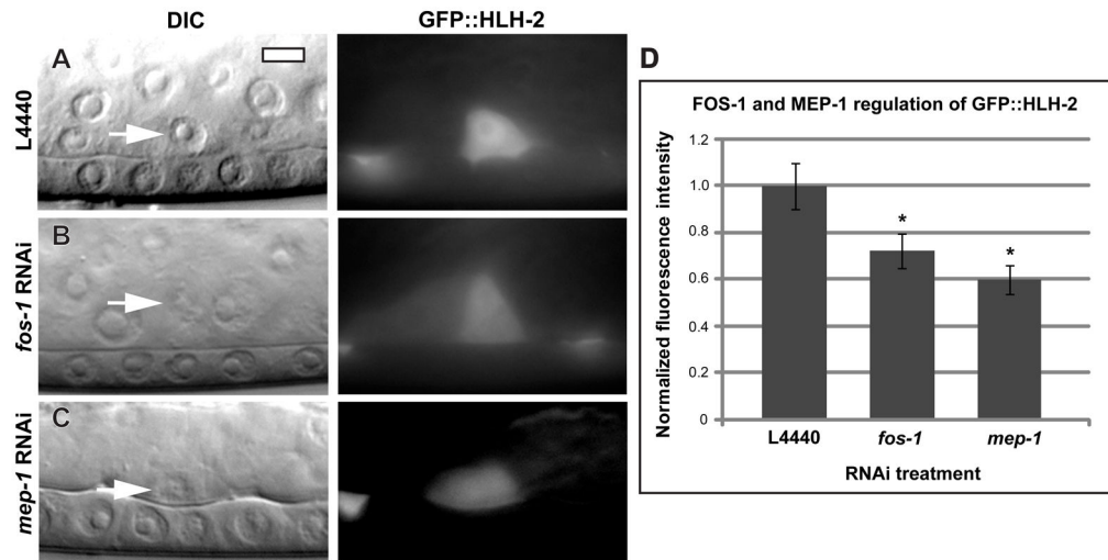
Figure 4. HLH-2 is partially regulated by FOS-1A and MEP-1
