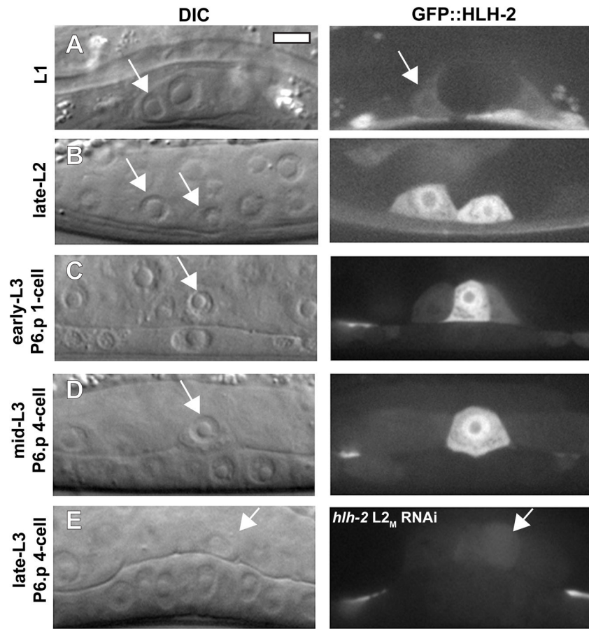
Figure 2. HLH-2 is expressed in the AC during specification and invasion
