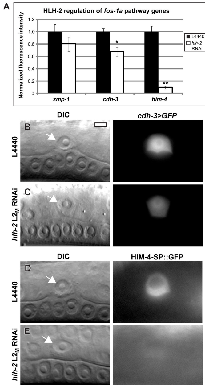
Figure 5. HLH-2 has parallel functions to FOS-1A in regulating AC-expressed genes
