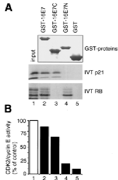
Figure 4. Analysis of binding sites in HPV-16 E7 proteins. (A) In vitro binding reactions with GST-16E7 mutants (1.5 \mu g) immobilized on glutathione-Sepharose and IVT p21 or IVT RB were performed, and the resulting protein complexes were visualized by Coomassie staining ( top ) and fluorography ( bottom ). Lane 1 represents 10% (IVT p21) or 20% (IVT RB) of the input. (B) Purified recombinant His-cyclin E/CDK2 complexes were coincubated with buffer ( \square ) or coincubated with His-p21 (10 ng, \blacksquare ) alone or with His-p21 preincubated with GST fusion proteins (300 ng; as indicated in A, lanes 2-5), and kinase assays were performed. The quantitation from PhosphorImager analysis is shown.
