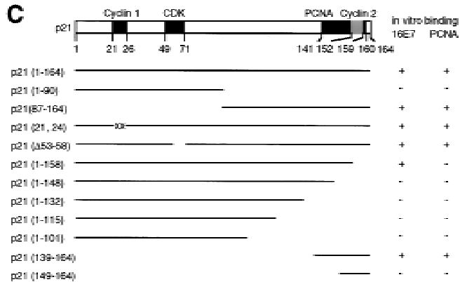
representation of p21 and summary of in vitro binding analyses with p21 mutants using purified and IVT proteins. The binding motifs for cyclin (cyclin 1), CDK, and PCNA are shown as solid boxes, the second cyclin binding motif (cyclin 2) overlapping the PCNA binding motif is shown as a shaded box.
