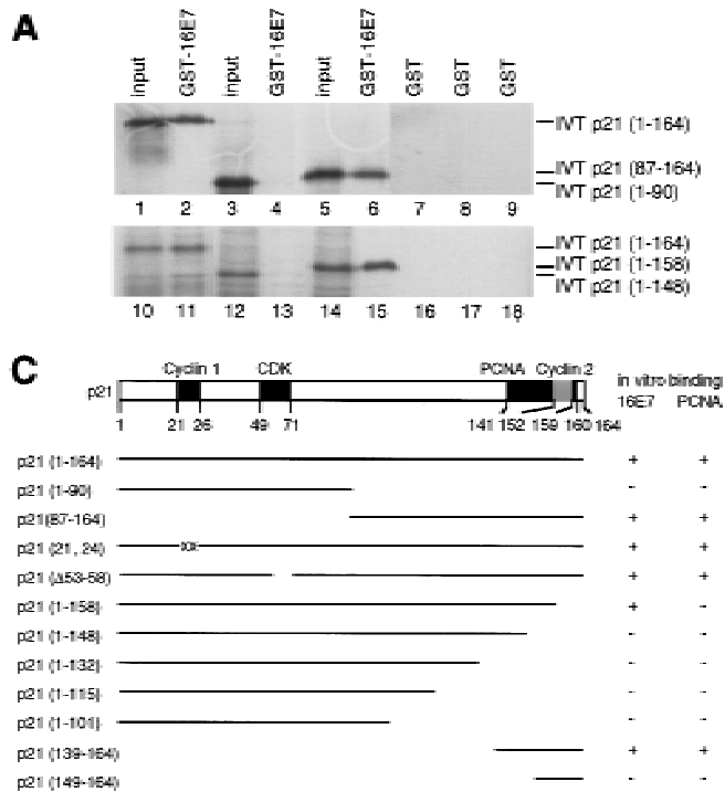
representation of p21 and summary of in vitro binding analyses with p21 mutants using purified and IVT proteins. The binding motifs for cyclin (cyclin 1), CDK, and PCNA are shown as solid boxes, the second cyclin binding motif (cyclin 2) overlapping the PCNA binding motif is shown as a shaded box.
