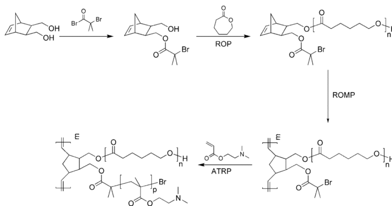
Scheme 18. Synthesis of a densely grafted amphiphilic brush block copolymer employing both the “grafting from” and “grafting through” strategies. 154
