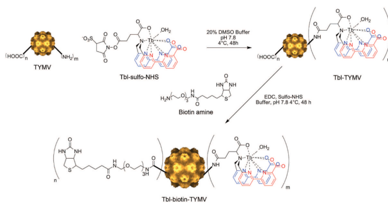
Scheme 70. Amidation strategies for viral functionalization. 404 (Reproduced with permission from ref 406. Copyright 2007 American Chemical Society).
