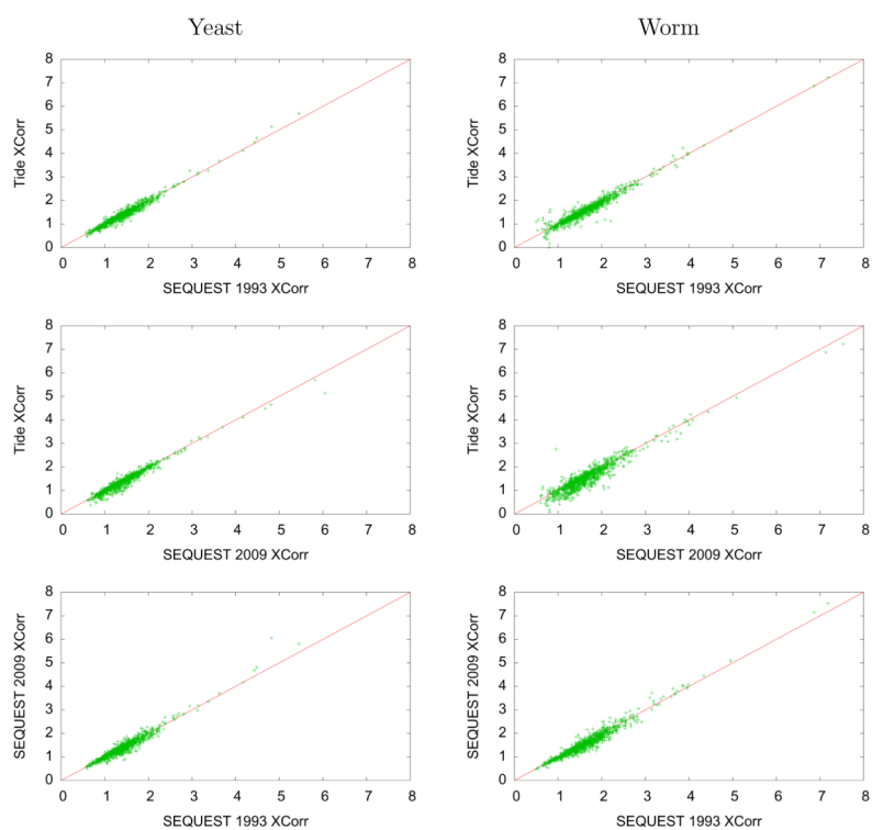
Figure 5. Comparison of X_{Corr} scores from Tide and from two versions of SEQUEST From two different data sets (yeast and worm), 100 spectra were selected at random for analysis by SEQUEST and by Tide. Searches were performed using a database of tryptic peptides from the corresponding organism, allowing up to two phosphorylations per peptide at occurrences of STY. The figure includes the top five PSMs per spectrum, as reported by SEQUEST. For each PSM, we plot the SEQUEST X_{Corr} versus the X_{Corr} computed by Tide. In the case of the bottom figures, we plot the SEQUEST 1993 X_{Corr} scores against those computed by SEQUEST 2009.
