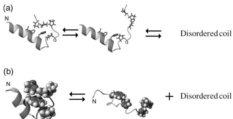
Fig. 7. Unfolding (melting) scenarios for Trp-cages with different degrees of intrinsic helix stability: (a) Trp-cage formation as Pro 17,18,19 docking onto a stable helix, (b) Trp-cage melting producing an unfolded ensemble retaining a measurable population of a residual hydrophobic cluster, a 'half-cage' structure.
