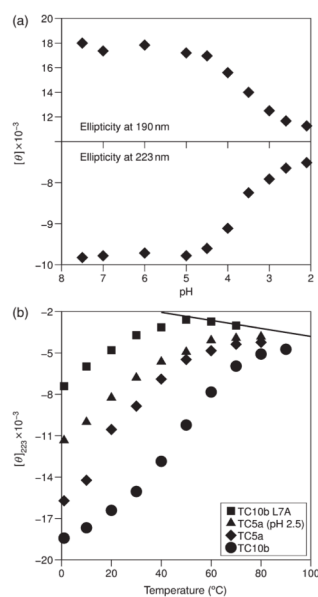
Fig. 5. (a) CD-monitored pH titration of fold stability for TC5a at 25°C; comparable effects were observed at both the maximum (190 nm) and the classical helix minimum (observed at 223.4 nm in this case). (b) Structure melting monitored at the 223 nm CD minimum; the unfolded baseline assumed for calculating fraction folded values (see Methods) is also given. The systems illustrated, in order of increasing stability, are: L7A-TC10b, TC5a at pH 2.5, TC5a at pH 7 and TC10b.
