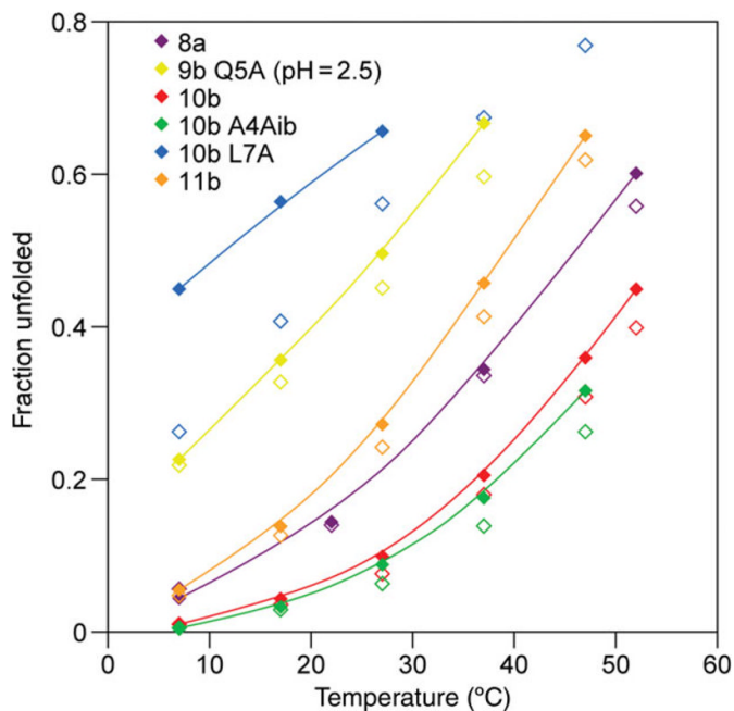
Fig. 3. ‘Cage’ (best fit lines through solid symbols) and ‘helix’ (open symbols) CSD melts, \chi_U versus T ( ^{\circ}\text{C} ), for representative mutants from Table I, with the exception of Q5A-TC9b (at pH 2.5), all melts were measured at pH 7. The (L7A)-mutant of TC10b illustrates the large deviations between helix and cage melts that can be observed for mutants with significantly destabilized cage structures. In more typical Trp-cage sequences, the helix measure yields \chi_U values that are only slightly smaller than the values based on the shifts that measure cage formation.
