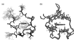
Fig. 4. Trp-cage NMR structure ensembles: (a) The TC10b structure ensemble (28 structures): heavy atoms are displayed for all residue side chains and the backbone, the hydrophobic cluster residues are shown in color in the version of this figure in the Supplementary data available at PEDS online. (b) An overlay of one member each of the TC10b and TC5b structure ensembles. All atoms are displayed for Tyr 3 , Trp 6 , Leu 7 , Pro 12 , Pro 18 and Pro 19 with only N, CA, C' shown for the remaining residues.
