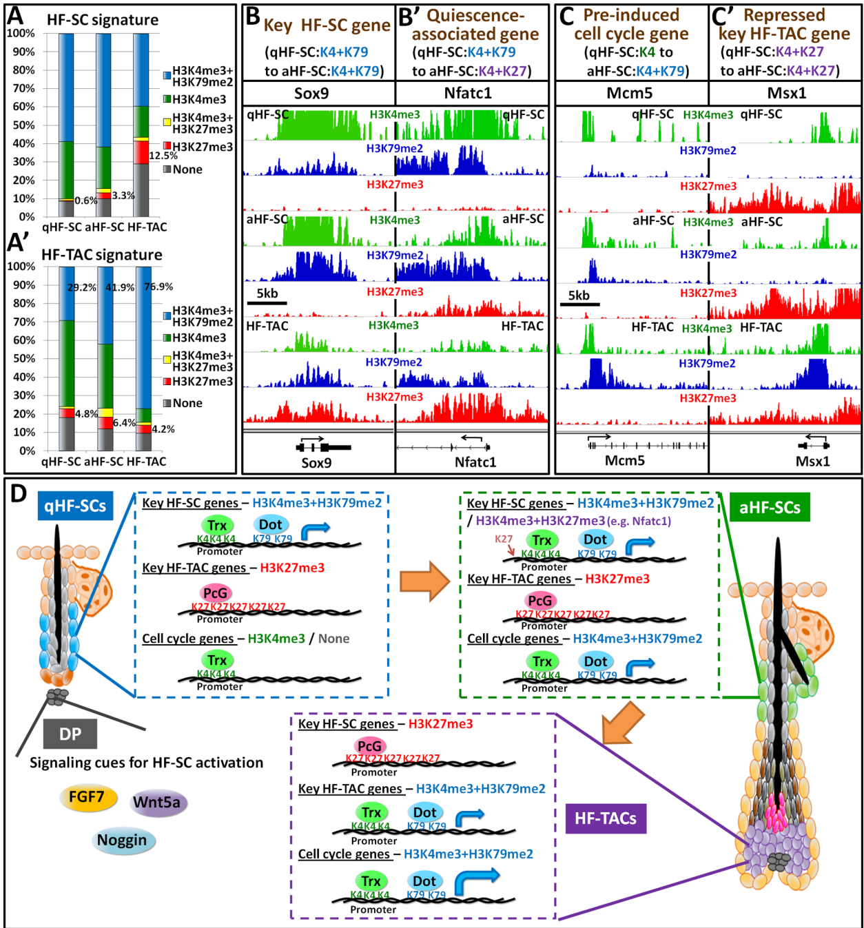
Figure 6. The Transition from Quiescent to Activated HF-SCs Maintains the Status of Many PcG-Regulated Genes While Activating Cell Cycle Genes Not Governed by PcG (A-A') Chromatin characteristics of HF-SC (A) and HF-TAC (A') signature genes are similar for quiescent and activated HF-SCs but distinct from HF-TACs. (B-B') Quiescent and activated HF-SC ChIP-seq profiles of key regulators of HF-SC maintenance (B) and quiescence (B'). All tracks are set to the same scale. Note chromatin changes in SC quiescence but not maintenance genes. (C-C') Cell cycle genes (e.g. Mcm5 in C), but not key matrix regulators (e.g. Msx1 in C') are pre-induced in aHF-SCs. ChIP-seq profiles from quiescent and activated HF-SC and HF-TAC chromatin. (D) Working model for PcG-mediated regulation in governing an irreversible fate switch. In qHF-SCs, key HF-TAC
