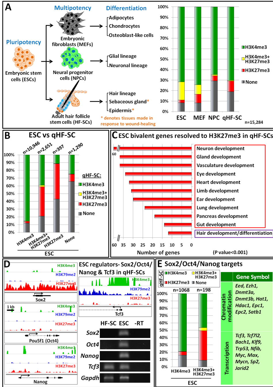
Figure 2. Genome-Wide Mapping of H3K4me3 and H3K27me3 Profiles in qHF-SCs (A) Global in vivo H3K4me3 and H3K27me3 patterns in qHF-SC chromatin, compared with published in vitro data on chromatin from cultured murine ESCs, MEFs and NPCs (Mikkelsen et al., 2007). In contrast to ESCs and MEFs, very few bivalent genes (yellow) were detected in qHF-SCs or NPCs. (B) Genes that in ESCs displayed one of four H3 methylation patterns (horizontal axis) and how this changes in qHF-SC chromatin. Each bar is normalized to 100% (n=number of ESC genes with each mark). Color-coding is for the qHF-SC genes and denotes the % of total genes within the ESC gene set that has either the same or a different mark in qHF-SCs. Green, H3K4me3; yellow, bivalent/dual marked with H3K4me3 and H3K27me3; red, H3K27me3; gray, neither mark. Note that most genes that
