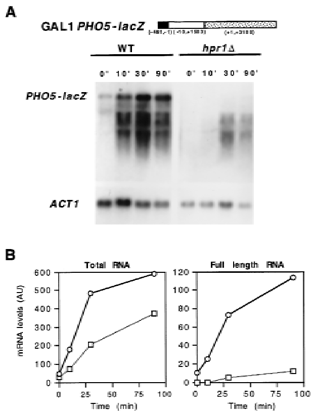
Figure 5. (A) Northern analysis of PHO5 mRNA. The DNA probe used for Northern analysis was the 1.5-kb EcoRI – PstI internal PHO5 fragment of pJDB207- PHO5 (Eco). Arbitrary units of mRNA were calculated according to the same standards for all experiments. (B) The mRNA values are given with respect to rRNA levels (see Materials and Methods). (○) Wild type; (□) hpr1 Δ. Other details as in Fig. 3.
