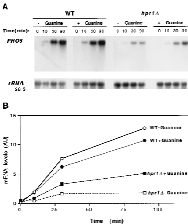
Figure 7. Transcription analysis of a yeast ORF in the presence of 6AU. Northern analysis (A) and kinetics of induction (B) of PHO5 mRNAs driven from the GAL1 promoter in the presence of 6AU with and without guanine are shown. The URA3 + wild-type and hpr1Δ strains transformed with pSch202 were obtained from overnight cultures in glycerol-lactate synthetic-complete media lacking tryptophan and uracil, and diluted in identical fresh media to an OD_{600} of 0.5 with 100 \mu g/ml of 6AU with and without 100 \mu g/ml of guanine. Galactose was added after 2 hr, and samples were taken for Northern analysis after different times, as specified. The mRNA values are given with respect to rRNA levels (B) (see Materials and Methods). Other details as in Fig. 3.
