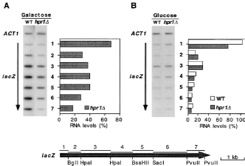
Figure 4. Transcriptional run-on analysis in wild-type and hpr1 Δ cells. Total RNA was isolated from wild-type and hpr1 Δ cells transformed with single-copy p416GAL1- lacZ plasmid under induction (A) and repression (B) conditions. Two percent-galactose or 2% glucose was added to yeast cultures in glycerol-lactate synthetic medium at an OD 600 of 0.05, 5 hr prior to the run-on analysis. The 0.6-kb internal ACT1 fragment and seven different DNA fragments (1–7) from the lacZ coding region were immobilized in hybond-N+ filters. The lacZ region covering each of the seven DNA fragments used is shown at the bottom. In all cases, the percentage of radiolabeled mRNA bound to each lacZ fragment was normalized with respect to their corresponding levels in galactose-grown wild-type cells, taken as 100% for each. The orientation of lacZ arrows indicates the direction of transcription. As negative control, we used DNA from Salmonella typhimurium (not shown).
