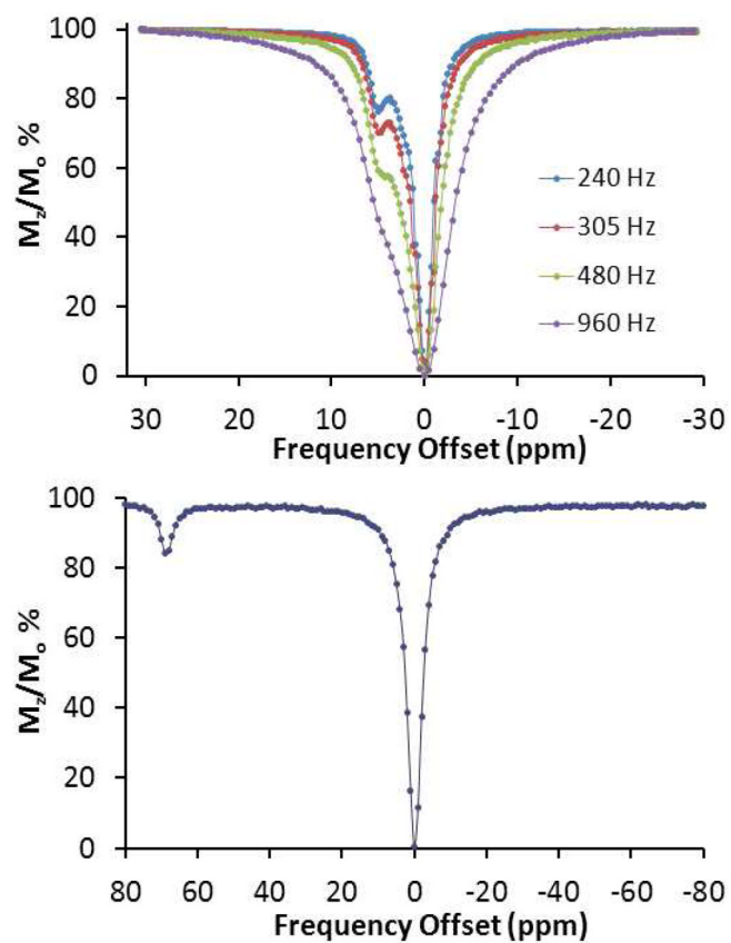
Figure 1. CEST spectra recorded at 400 MHz of (top): 4 mM [Fe(L2)] 2+ , pH 7.0 at 25 °C with B_1 as shown and 4 s presaturation pulse and (bottom): 8 mM [Fe(L1)] 2+ 20 mM HEPES pH 6.8, 100 mM NaCl, 37 °C, with B_1 = 960 Hz, 4 s.
