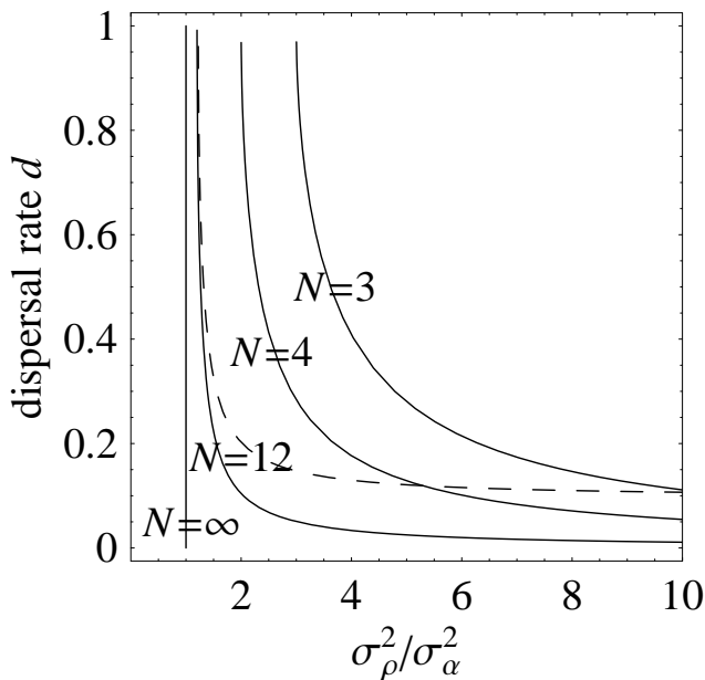
Figure 1 Threshold combinations of values of \sigma_\rho^2 / \sigma_\alpha^2 and d for disruptive selection. The lines are the thresholds for different values of N . Branching is favored for sets of values in the top right corner delimited by these lines. The dashed line shows the thresholds for N = 12 obtained with the approximation K = 0 .
