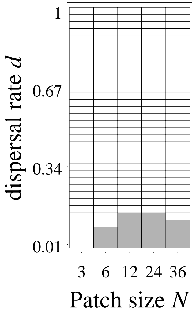
Figure 2 Cases of global instability. The shaded area is the set of parameter values for which some mutants invade despite local non-invasibility of the candidate ESS z^* . This figure is obtained from computation of R_m for \delta up to 2.187.
