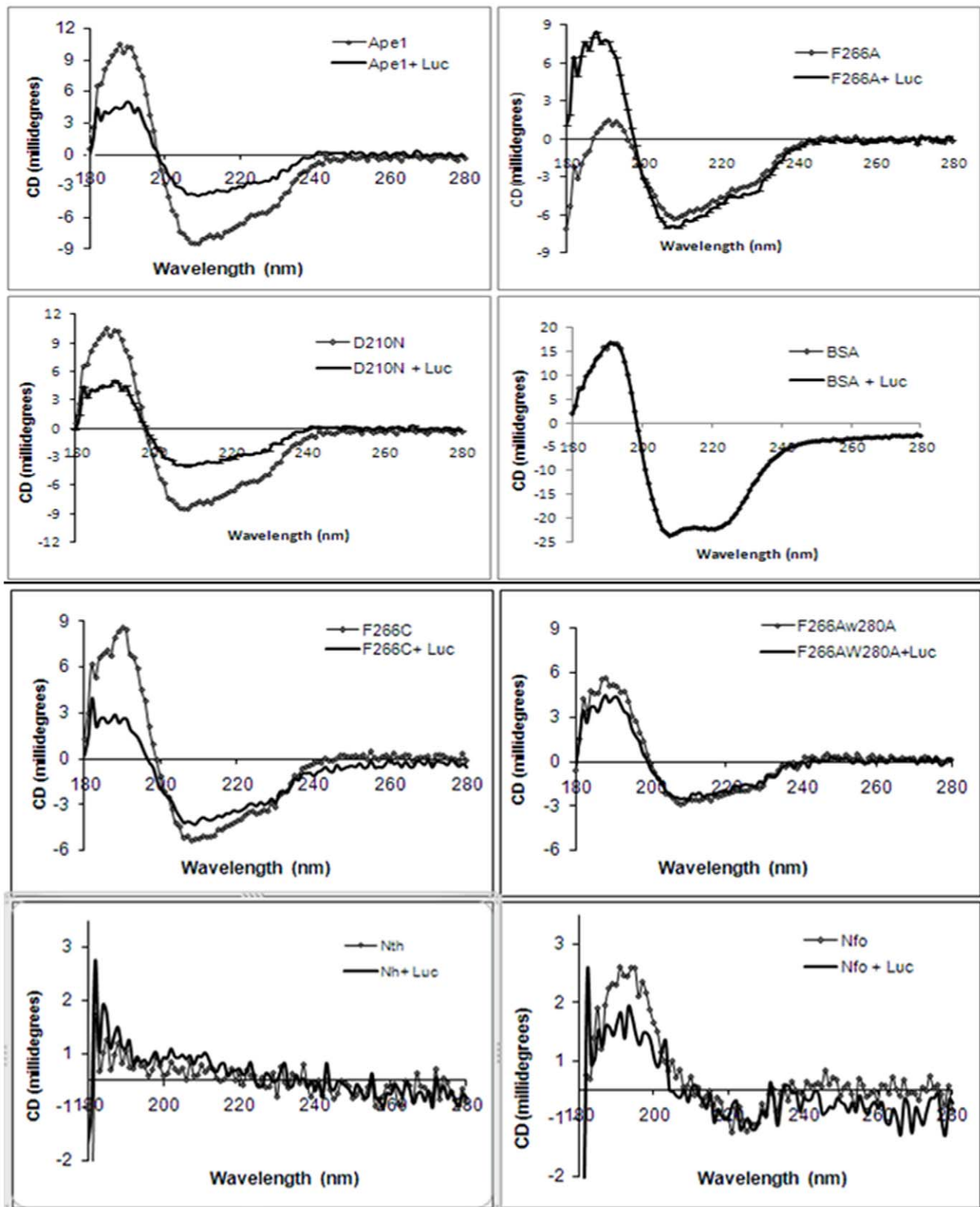
Figure 13. Lucanone does not alter conformation of double hydrophobic site APE1 mutant, human Nth and bacterial Nfo proteins. CD spectra of APE1 and its mutants in presence of lucanone. APE1- hydrophobic site mutant proteins F266A/C, F266A/W280A, active site mutant D210N and non-related BSA protein or human Nth or E.coli Nfo(10 mg/ml), 50 \mu l (500 \mu g) (14 \mu M) in APE1 buffer (50 mM HEPES, 150 mM KCl, 5 mM MgCl_2 ), was mixed with lucanone (1 mg/ml), 50 \mu l (50 \mu g) (140 \mu M), incubated at 37°C for 60 min and far UV-CD spectra with specifications.
