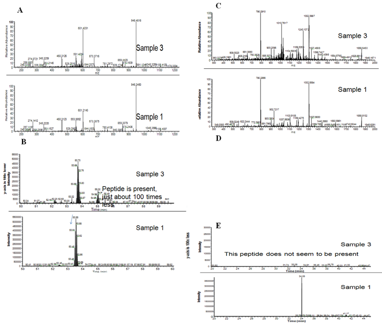
Figure 9. Identification of an approximate lucanthone cleavage site in APE1. LC/MS/MS identification of APE1 fragment after treatment with 100 \mu M of lucanthone for 2 h at 37°C. The data were analyzed with Inspect. A). Peptide aa64–73 analysis of 35.5 Kda (Sample 1) and 25 kDa (Sample 3). B). Elution profile of peptide aa64–73 in sample 1 and 3. C). Peptide aa282–299 analysis of 35.5 Kda (Sample 1) and 25 kDa (Sample 3). D). Peptide aa53–63 analysis of 35.5 Kda (Sample 1) and 25 kDa (Sample 3). E). Elution profile of peptide aa53–63 in sample 1 and 3. doi:10.1371/journal.pone.0023679.g009
