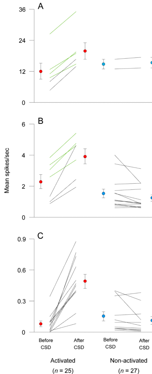
Figure 5. Firing rate before and after CSD in activated and non-activated central trigeminovascular neurons. Individual plots and mean \pm SEM values are shown for activated (left, red circles) and non-activated units (right, blue circles). A neuron was considered activated when its mean firing rate after CSD exceeded its mean baseline activity by 2 standard deviations of that mean over a period >10 min as shown in Fig. 4. (A) Neurons exhibiting high rate of baseline activity ( 12.09 \pm 3.09 ; range 5–26 spikes/sec) increased their firing rate to 19.85 \pm 3.19 spikes/sec (65%) after CSD. (B) Neurons exhibiting medium rate of baseline activity ( 2.3 \pm 0.46 ; range 0.6–4 spikes/sec) increased their firing rate to 3.92 \pm 0.49 spikes/sec (75%) after CSD. (C) Neurons exhibiting low rate of baseline activity ( 0.08 \pm 0.03 ; range 0–0.4 spikes/sec) increased their firing rate to 0.49 \pm 0.07 spikes/sec (600%) after CSD.
