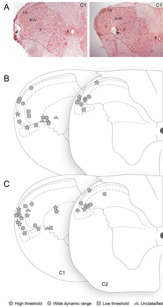
Figure 2. Localization of lesions marking the recording sites in the dorsal horn (1 neuron per rat). (A) Photomicrographs showing lesion (pointed by arrowheads) in laminae I (left) and V (right) of the first cervical segment (C1). (B) Mapping of 25 lesions marking the locations of activated neurons. (C) Mapping of 27 lesions marking the locations of non-activated neurons. Neuronal type is indicated by the key at bottom of figure.
