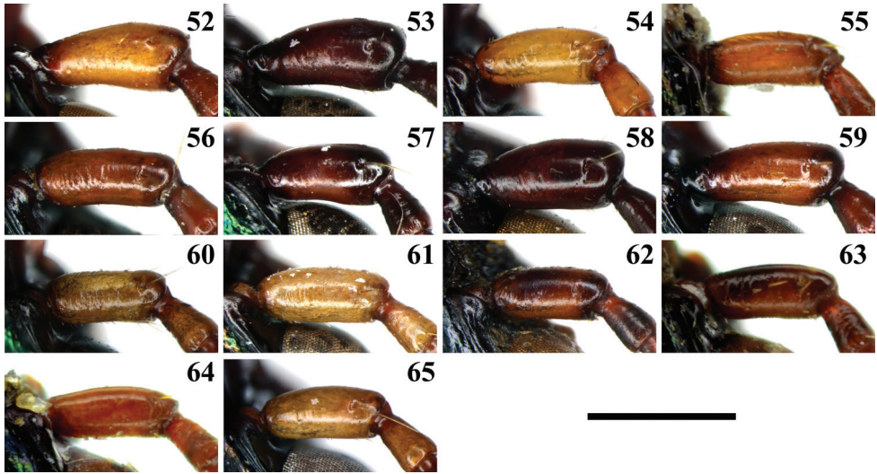
Figures 52–65. Antennomere 1 of Chlaenius ( Lithochlaenius ) species 52 C. chuanqianensis sp. n., holotype 53 C. linwensini sp. n., holotype 54 C. propeagilis sp. n., holotype 55 C. agilis Chaudoir, holotype 56 C. formosensis Lorenz, CCCC 57 C. leishanensis Kirschenhofer, IZCAS 58 C. noguchii Bates, IZCAS 59 C. wrasei Kirschenhofer, IZCAS 60 C. agiloides Jedlička, IZCAS 61 C. rambouseki Lutshnik from Ussuri region, IZCAS 62 C. anchomenoides Bates, paratype 63 C. nuristanus Jedlička, paratype 64 C. nuristanus a. rubridipes Jedlička, paratype 65 C. rambouseki Lutshnik from Taiwan, CCCC. Scale line = 1.0 mm.
