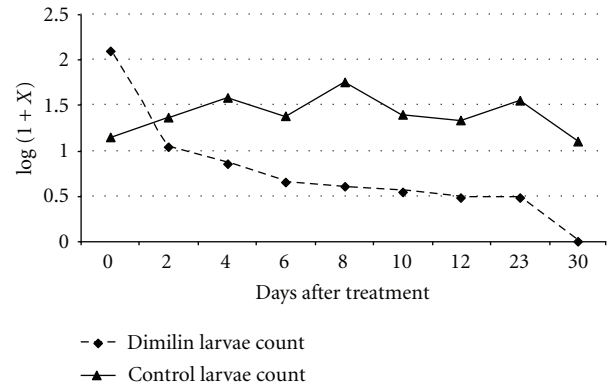
FIGURE 1: Mean anopheline larvae count in Dimilin granules-treated rice field.
