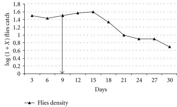
FIGURE 5: Mean housefly count over time. Note. The arrow marks the treatment day.
