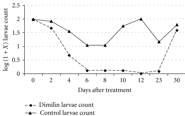
FIGURE 3: Mean anopheline larvae count in Dimilin powder-treated sites over time.
