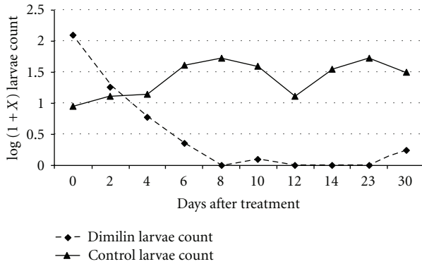
FIGURE 4: Mean culicine larvae count over time in Dimilin Tablet treated pits.
