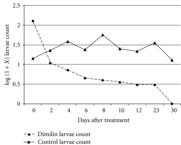
FIGURE 2: Mean culicine larvae count in Dimilin granules-treated rice plots.
