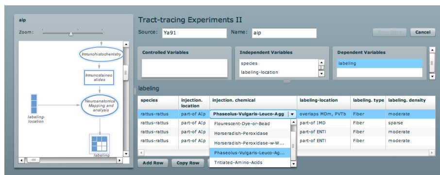
Figure 5 KEFED data form for a tract-tracing experiment. The KEFED editor showing the data form derived from the tract-tracing model. The data entry table (spreadsheet) view is generated automatically by tracing the data dependencies in the model design. This insures that the entire relevant context for measurements is captured. This form shows data entered from a curated experiment [62].
