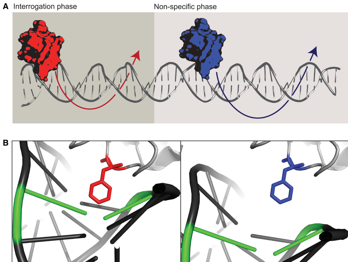
Figure 7. The glycosylase search model. (A) Glycosylases rotate around the DNA molecule interrogating bases (red) or by non-specific rotation when interrogation does not occur (blue). (B) A structural model of Fpg glycosylase undergoing slow diffusion, sampling for damage using a wedge amino acid (red) or fast diffusion without intrahelical interrogation (blue) (PDB 2F5O).
