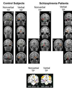
Figure 1. Illustration of localization of task-specific and hemisphere-specific hippocampal activity during nonverbal and verbal variants of a transverse-patterning (TP) task in four nonpatient and four patient individuals. Upper panel: MEG-based localization (each row is one subject). Controls showed consistent lateralization as a function of task. Patients showed less consistent activation. Lower panel: fMRI-based localization, in which blue arrows point to hippocampal activation, lateralized as a function of task (combined analysis for three nonpatients and four patients). Figure is adapted from Hanlon et al. (2007).
