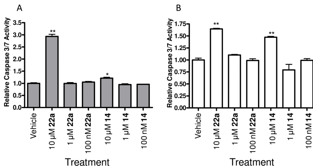
Figure 7. Inhibition of PLD2 leads to increased apoptosis in MDA-MB-231 cells compared with minimal effect of PLD1 inhibition. MDA-MB-231 cells were cultured in the presence of PLD inhibitor for 48 hours after which time Caspase 3 & 7 activity was measured. A. MDA-MB-231 cells cultured in the presence of 10% FBS were fairly resistant to PLD inhibitor treatment ( 14 or 22a ) with only 10 μM 22a treatment leading to a significant increase in Caspase 3 & 7 activity compared to vehicle control. B. MDA-MB-231 cells cultured under serum free conditions had increased Caspase 3 & 7 activity upon 10 μM PLD inhibitor treatment as compared to the vehicle control. * p < 0.05 , ** p < 0.01 . Data is representative of three independent experiments. Error bars show standard error of the mean for triplicate measurements.
