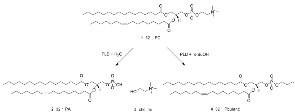
Figure 1. PLD catalyzed the hydrolysis of phosphatidylcholine 1 (PC) into phosphatidic acid 2 (PA) and choline 3 . In the presence of a primary alcohol, typically n -butanol, PLD catalyzes a unique transphosphatidylation reaction to produce phosphatidylbutanol 4 .
