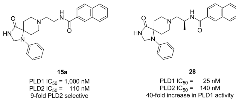
Figure 8. Structures and activities of PLD2 preferring inhibitor 15a and impact of a chiral ( S )-methyl group providing 28 and a 40-fold increase in PLD inhibitory activity.
