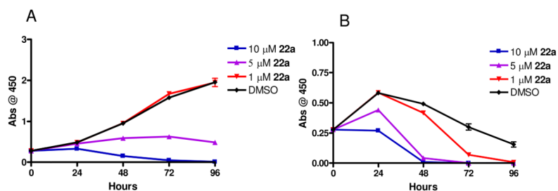
Figure 6. Inhibition of PLD2 leads to a time dependent decrease in proliferation of MDA-MB-231 cells. MDA-MB-231 cells were cultured in the presence of PLD inhibitor and cell viability was assayed using WST-1 cell proliferation reagent over 96 hours. A. MDA-MB-231 cells cultured in the presence of 10% FBS showed a dose dependent attenuation of cell proliferation over time. Cultures with 10 and 5 μM 22a treatment led to a significant decrease in cell proliferation while 1 μM inhibitor had no effect. B. MDA-MB-231 cells cultured in the absence of serum had a more pronounced response to PLD inhibition with all concentrations of the PLD2 selective compound significantly decreasing cell proliferation in a dose and time dependent manner. Data is representative of three independent experiments. Error bars show standard error of the mean for triplicate measurements.
