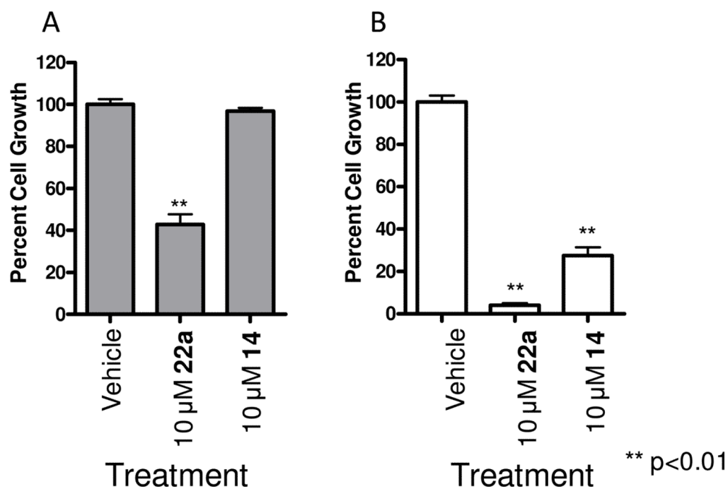
Figure 5. Inhibition of PLD2 with 22a leads to decreased proliferation of MDA-MB-231 cells. MDA-MB-231 cells were cultured in the presence of PLD inhibitor for 48 hours after which cell viability was assayed using WST-1 cell proliferation reagent. A. MDA-MB-231 cells cultured in the presence of 10% FBS were fairly resistant to PLD inhibitor treatment with only 10 μM 22a treatment leading to a significant decrease in cell proliferation. B. MDA-MB-231 cells cultured under serum free conditions had a more pronounced response to PLD inhibition with both PLD1 ( 14 ) and PLD2 ( 22a ) selective compounds significantly decreasing cell proliferation. n=3. Error bars show standard error of the mean for triplicate measurements.
