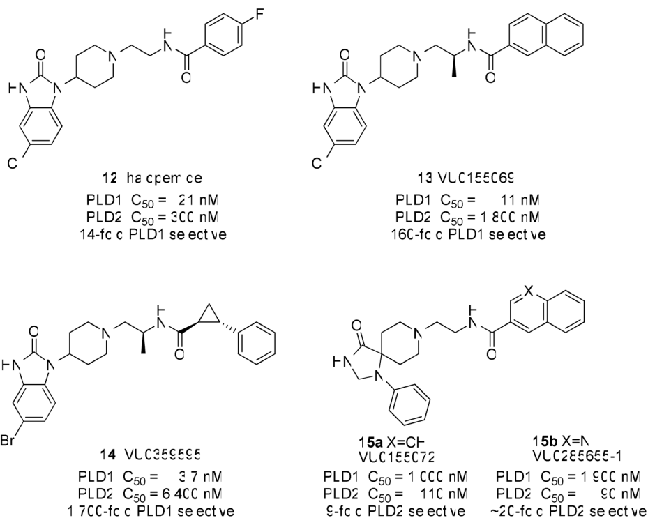
Figure 3. Structures and activities of haloperamide 12 and isoform-selective PLD inhibitors 13 and 14 (PLD1 selective) and 15a–b (PLD2 preferring).
