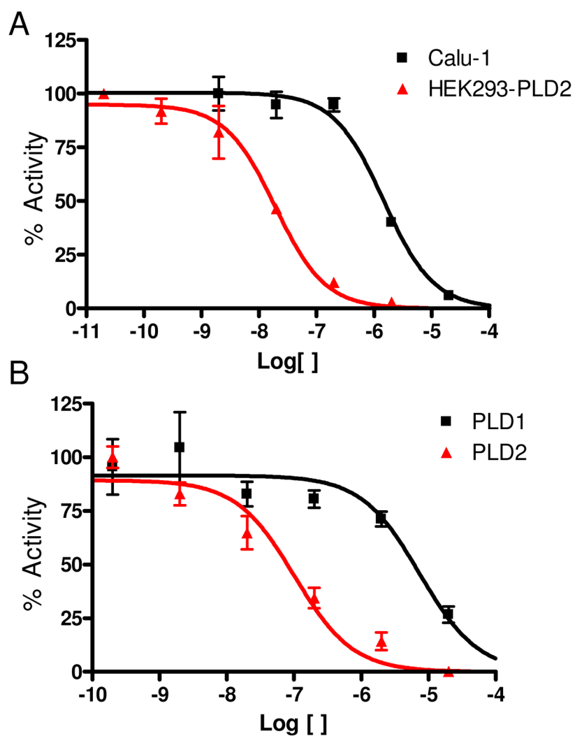
Figure 4. Concentration-Response-Curves (CRCs) for A) cellular PLD1 ■ (Calu-1) assay and PLD2 ▲ (HEK293-gfpPLD2) assay and B) biochemical inhibition assay CRCs with purified ■ PLD1 and ▲ PLD2 highlighting the unprecedented 75-fold PLD2 versus PLD1 selectivity for 22a in both PLD assays. Error bars show standard error of the mean for triplicate measurements.
