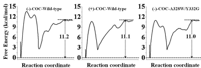
Figure 4. Free energy profiles for the formation of prereactive complex for wild-type BChE binding with (-)-cocaine (left), wild-type BChE binding with (+)-cocaine (middle), and the A328W/Y332G mutant binding with (-)-cocaine (right).
