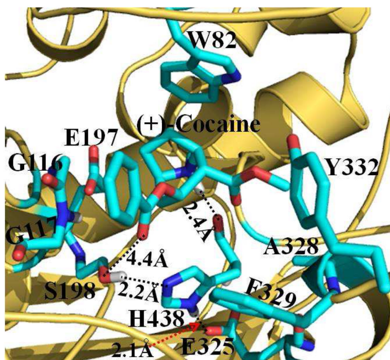
Figure 2. MD-simulated nonpreactive complex structure for (+)-cocaine binding with wild-type BChE. BChE is shown as gold ribbon. (+)-cocaine molecule and residues of BChE within 5 Å around (+)-cocaine are shown in the stick style and colored by the atom type. The distances from the proton at the cationic head of (+)-cocaine to the backbone oxygen atom of residue H438 and from the carbonyl oxygen at the benzoyl group of (+)-cocaine to the OG atom at the hydroxyl group of residue S198 are represented as dashed lines and labeled. Labeled also are the hydrogen bonds formed within the catalytic triad S198-H438-E325 of BChE.
