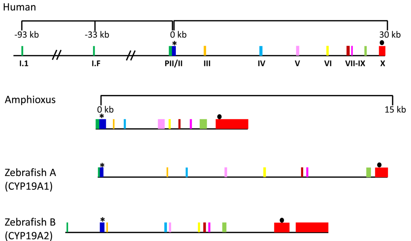
Figure 2. Comparison of CYP19 genes in amphioxus, human and zebrafish
