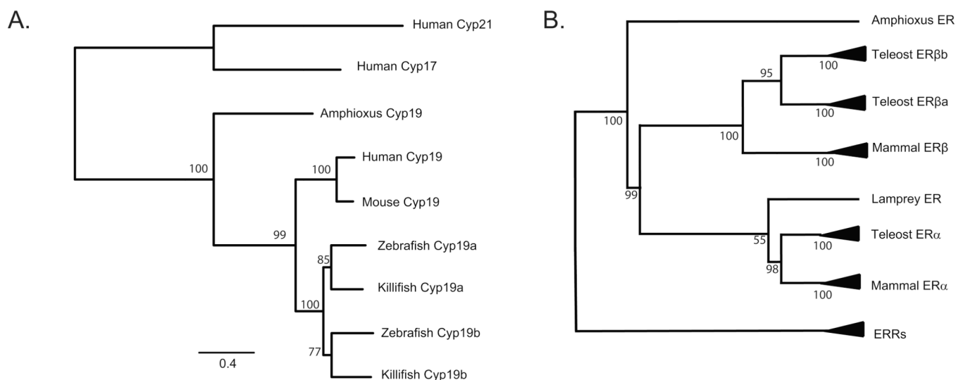
Figure 1. Phylogenetic trees of (A) aromatase and (B) ER proteins
