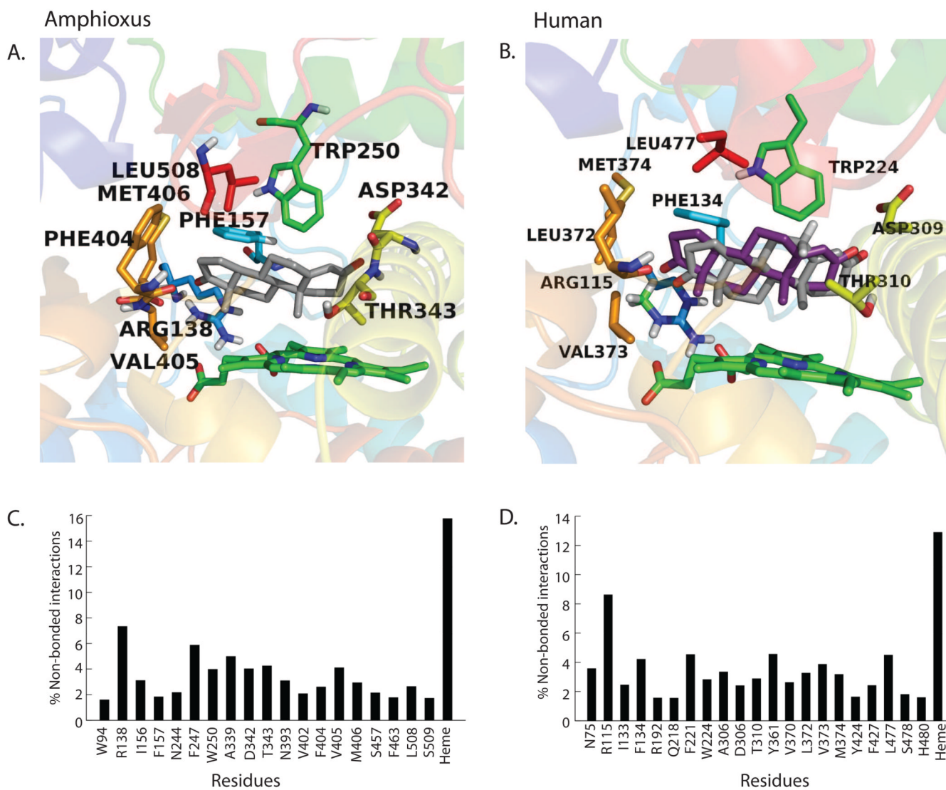
Figure 4. Homology model of androstenedione docked within the active site of aromatase in (A) amphioxus and (B) human and plot of non-bonded interactions in (C) amphioxus and (D) human See sections 2.3 and 3.5 for detailed methods and results describing evolutionarily conserved residues. Also, compare with conserved residues identified by sequence alignment (Fig. 3; section 3.3.2).
