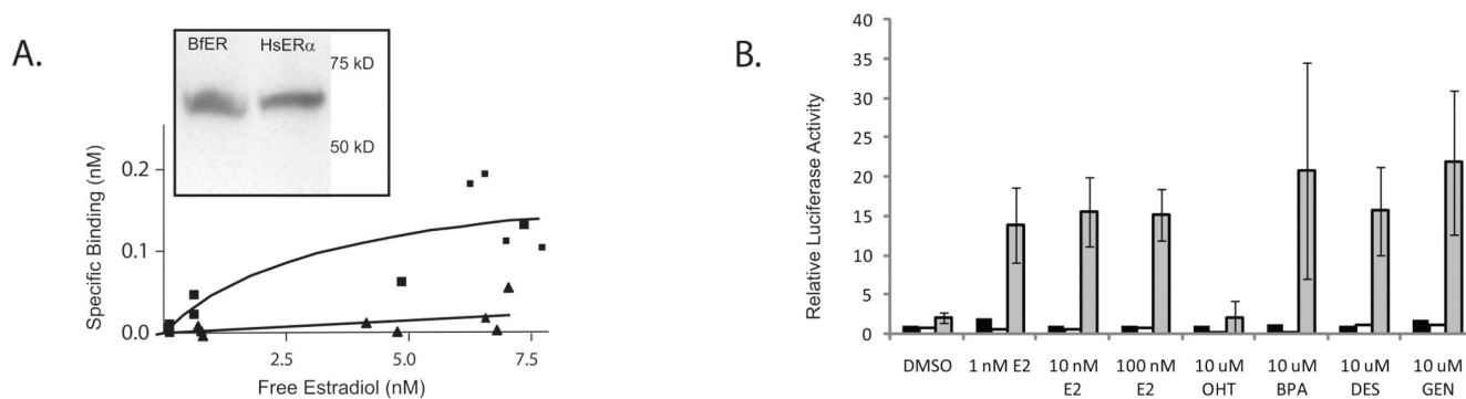
Figure 5. Functional comparison of amphioxus ER through binding experiments and cell-based reporter assays
