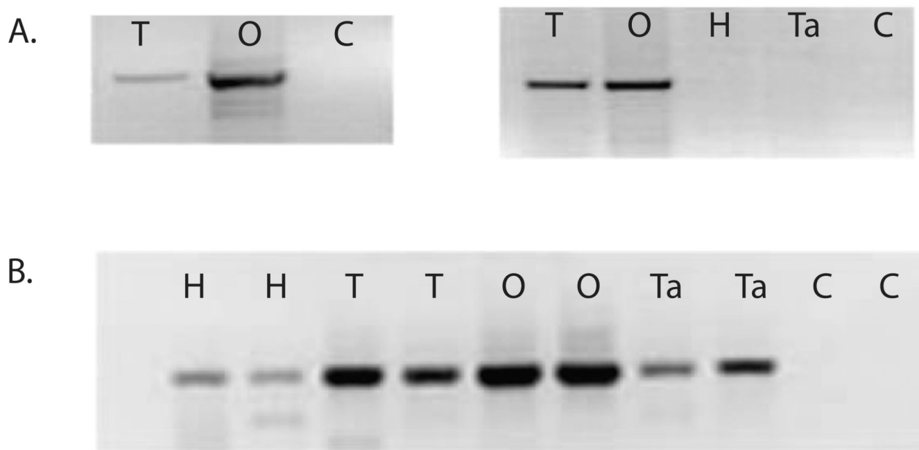
Figure 6. Tissue-specific expression of (A) CYP19 and (B) ER mRNAs in amphioxus, as determined by semiquantitative RT-PCR analysis
