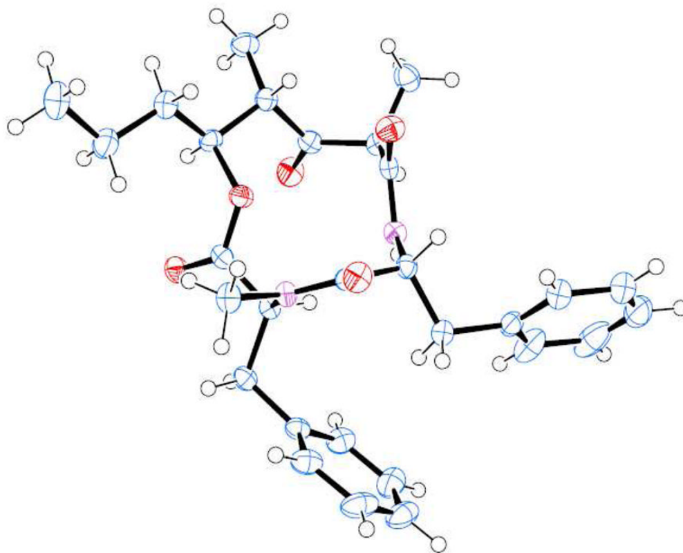
Figure 2. ORTEP drawing of Compound 14
