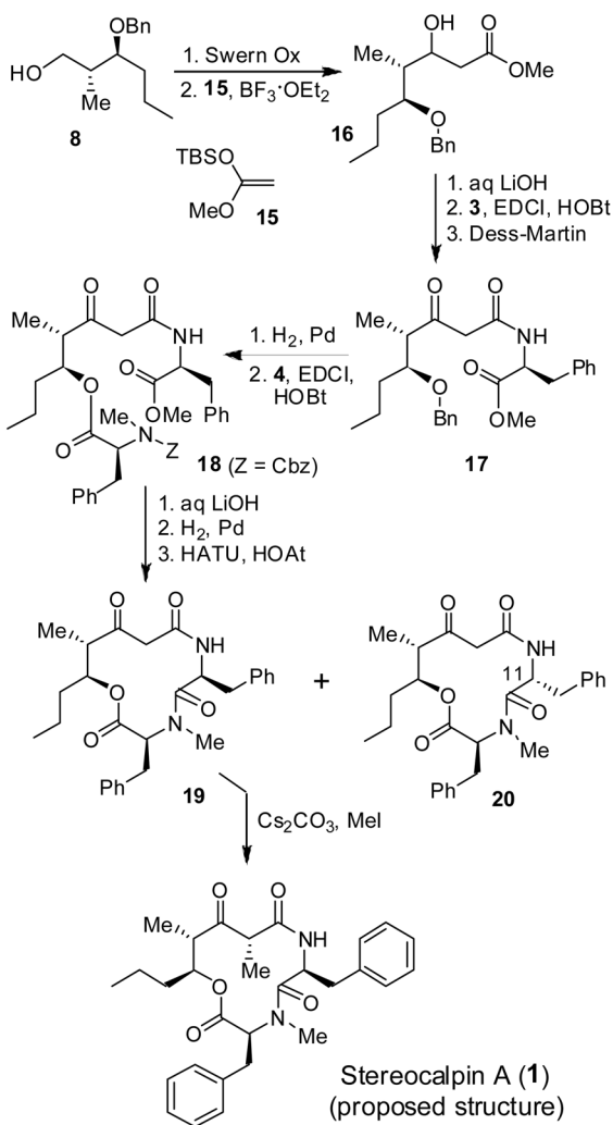
Scheme 3. Synthesis of Stereocalpin A (proposed structure)
