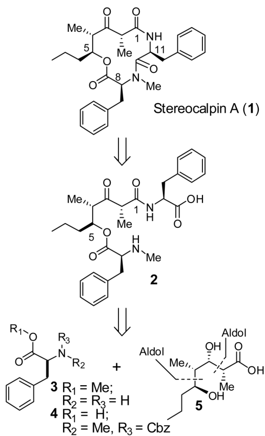
Figure 1. Retrosynthesis of Stereocalpin A.
