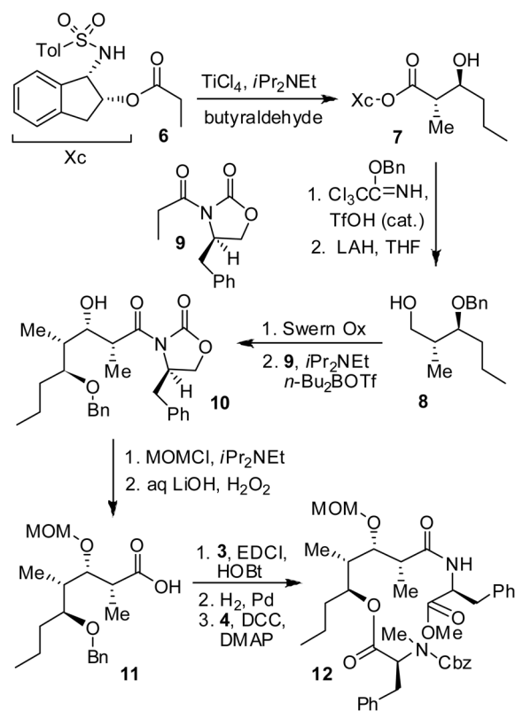
Scheme 1. Synthesis of Cyclization Precursor 12
