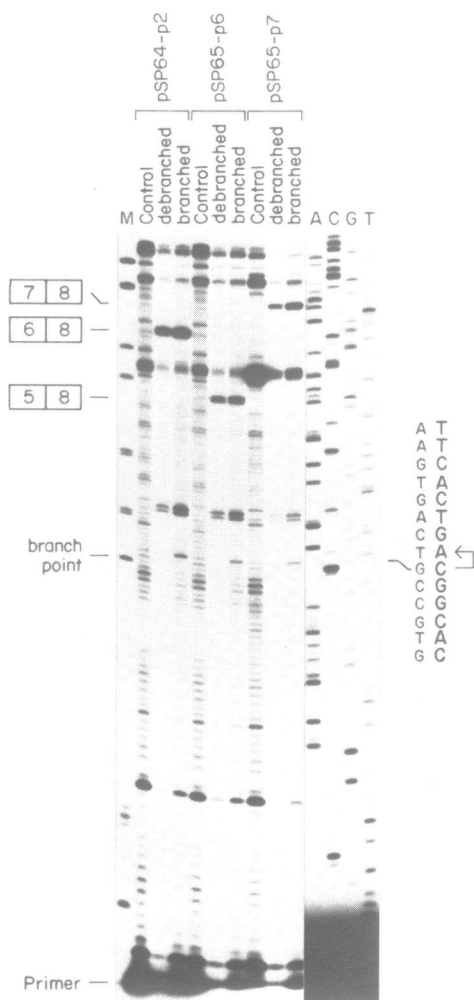
Figure 6. A single branch point is utilized during the splicing of exon five, six or seven to exon eight. Precursors derived from pSP64-p2 linearized with Sall, pSP65-p6 linearized with Sall, and pSP65-p7 linearized with HindIII were spliced for 2 h in vitro . The in vitro processing products were analyzed by primer-extension using a 32 P-labelled oligonucleotide primer specific for sequences in the middle of exon 8. Half of the processed RNA was treated with debranching extract prior to primer-extension analysis. Position of the primer extension products corresponding to splice products and intermediates are indicated. The primer extension products were separated on a 8% denaturing polyacrylamide gel and electrophoresed in parallel with dideoxy sequencing reactions performed using single stranded M13 templates primed with the same 32 P-labelled oligonucleotide primer to the right. The sequences corresponding to positions -18 through -31 nucleotides upstream from the 3' splice site and the corresponding branch nucleotide are indicated.
