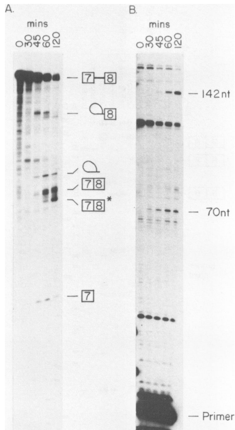
Figure 5. In vitro splicing of exon seven to exon eight (skeletal muscle-type splice). (Panel A) Time course (min) of formation of spliced products from transcripts terminating at the HindIII site of plasmid pSP65-p7. The ^{32}\text{P} -RNA products were separated in 4% denaturing polyacrylamide gels. Schematic representation of products are indicated; the boxes represent exon sequences and the lines intron sequences. Due to the presence of a 3' exonuclease activity the splice product appears as two bands and is indicated with an asterisk. (Panel B) The in vitro processing products shown in panel A were analyzed by primer-extension using a ^{32}\text{P} -labelled oligodeoxynucleotide primer specific for sequences in exon 8. Position of primer extension products corresponding to splice products and intermediates are indicated.
