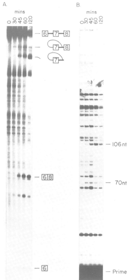
Figure 4. In vitro splicing of exon six to exon eight (fibroblast-type splice). (Panel A) Time course (min) of formation of spliced products from transcripts terminating at the SalI site of plasmid pSP65-p6. The ^{32}\text{P} -RNA products were separated in 4% denaturing polyacrylamide/ gels. Schematic representation of products are indicated; the boxes represent exon sequences and the lines intron sequences. (Panel B) The in vitro processing products shown in panel A were analyzed by primer-extension using a ^{32}\text{P} -labelled oligodeoxynucleotide primer specific for sequences in exon 8. Positions of primer extension products corresponding to splice products and intermediates are indicated.
