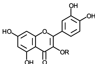
Flavonols Quercetin (R=H) and Quercetin-glycosides (R=sugar moiety)
