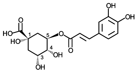
Hydroxycinnamic acids 5-Caffeoylquinic acid (Chlorogenic acid)
