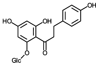
Dihydrochalcones Phloretin-2'-glucoside (Phloridzin)
