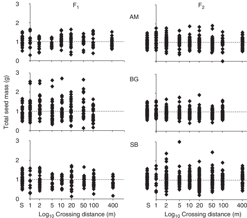
Figure 4 Variation in RP of F_1 and F_2 plants derived through self- (S) and cross-pollination in the three populations. Variation in seed number and total seed mass was very similar and therefore only total seed mass is shown.
