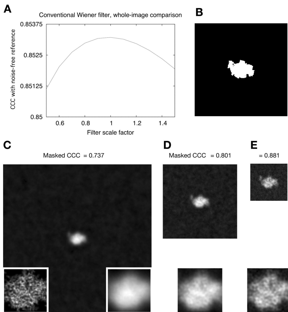
Figure 2. Image restoration of a synthetic single-particle image using a conventional Wiener filter
