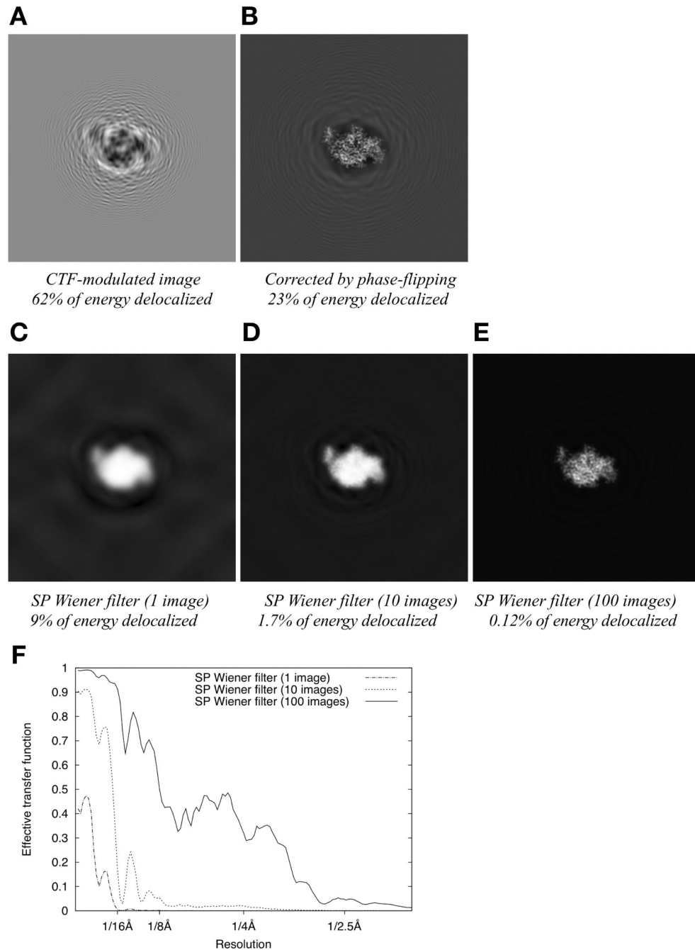
Figure 3. re-localization of signal intensity by single-particle Wiener filtering applied to a defocus series of images
