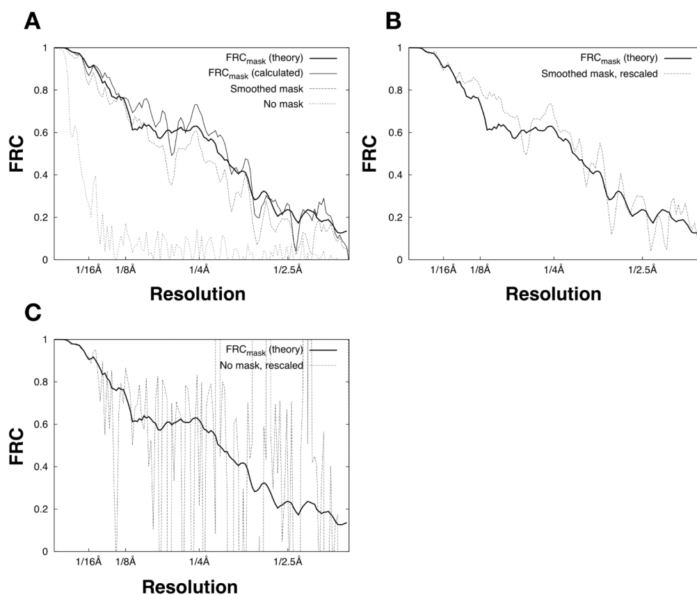
Figure 5. Estimation of the PSSNR from masked FRC calculations
