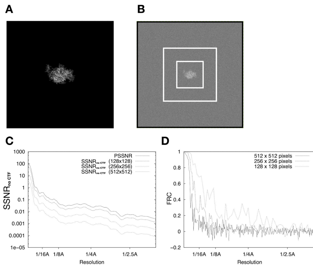
Figure 1. FRC calculations for isolated single particles depend on image size
