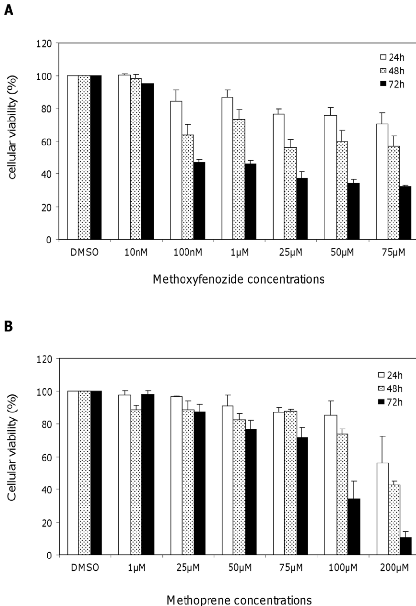
Figure 1. Methoxyfenozide and methoprene toxicity to Sf9 cells. Cell viability was followed by the MTT test at 24, 48 and 72 h post-treatment of Sf9 cells by methoxyfenozide (A) or methoprene (B). Data are the mean of three independent experiments with SE. doi:10.1371/journal.pone.0025708.g001
