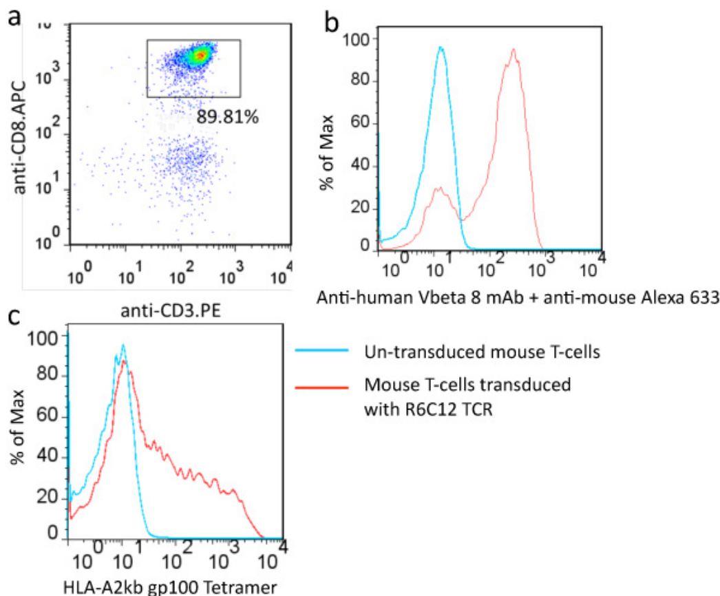
Figure 2. Example of successful isolation and transduction of mouse T-cells. (a) CD8 T-cells were isolated from splenocytes using CD8a + T Cell Isolation Kit (Miltenyi Biotec) and stained with anti-CD3e and anti-CD8a antibodies. Isolated CD8 T-cells were transduced with R6C12 TCR specific for human gp100:209 -217 4 peptide and stained with anti-human Vbeta 8 antibody (b) and HLA-A2kb gp100 tetramer (c).
