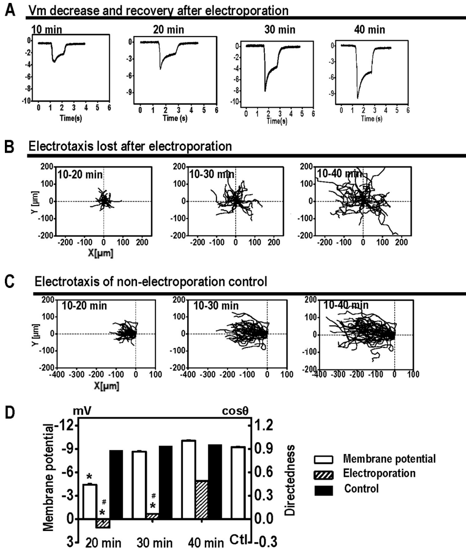
FIG. 4. Electroporation depolarizes membrane potential ( V_m ) and abolishes electotaxis. (A) Representative V_m measured at pH 6.5 after electroporation. The moment of electroporation was set as time zero. (B) Electroporated cells lost the electotactic response, which showed some degree of recovery 30 min later (see video S6 in the supplemental material). (C) Control cells showed robust electotaxis. (D) Loss of electotaxis correlated well with V_m . When V_m recovered, electotaxis recovered significantly. Control, V_m in control cells not electroporated. The EF was 12 V/cm. *, P < 0.001 compared to that of cells not being electroporated; #, P < 0.001 compared to that of cells after 40 min of recovery following electroporation.
