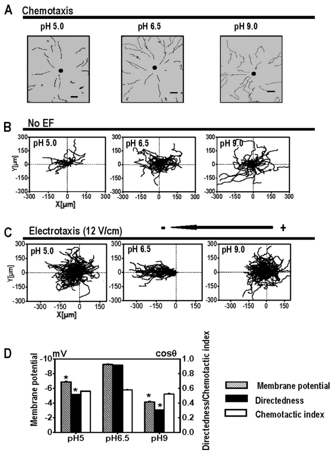
FIG. 2. Extracellular pH plays different roles in chemotaxis and electrotaxis in Dictyostelium cells. (A) cAMP gradients were formed from the tip of a micropipette filled with 10 \mu\text{M} cAMP. Trajectories of cell migration toward cAMP in DB with different pH values are indicated. Dark spots represent the position of the micropipette. Scale bar, 20 \mu\text{m} . (B) Cell migration in random directions under control conditions without an EF although cells were bathed in DB with different pH values as indicated. (C) Cell migration trajectories in which the start point of each cell is set as the origin. Cells migrated cathodally in a pH of 6.5 in an EF. However, directed cell migration was significantly impaired under acidic (pH 5.0) or alkaline (pH 9.0) conditions. (D) The effects of extracellular pH on electrotaxis in Dictyostelium cells correlate with the effects on V_m . Dictyostelium cells bathed in pH 6.5 showed a greater V_m than that of the cells in pH 5.0 or pH 9.0 and significantly better electrotaxis. The changes in pH and corresponding changes in V_m did not significantly affect the chemotaxis (chemotactic index). *, P < 0.001 compared to that in pH 6.5.
