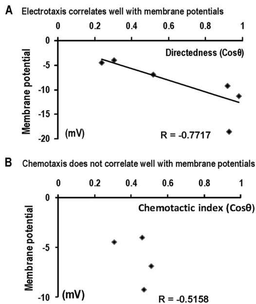
FIG. 5. Significant correlation is between V_m and electrotaxis but not chemotaxis. (A) Scatter plot shows electrotactic directedness and resting membrane potential ( r = -0.77 ). The best-fit line is shown. (B) Scatter plot shows chemotactic index and membrane potential ( r = -0.51 ).
