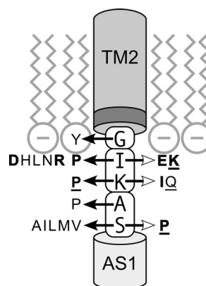
FIG. 9. Signaling properties of control cable lesions. The cartoon depicts the inner leaflet of the cytoplasmic membrane and the portions of the TM2 and AS1 helices that adjoin the control cable. The darker segment at the cytoplasmic end of TM2 denotes the aromatic belt residues (W211, F212) that partition at the lipid tail-head group interface. Amino acid replacements in the control cable that impair (lightface type) or abrogate (boldface type) signaling function are indicated by horizontal arrows: white arrowheads denote lesions with REP-mimic properties, and black arrowheads denote lesions with ATT-mimic properties. Underlined replacements produce some, but not all, of the signaling characteristics of ATT- or REP-mimic defects. Proline replacements, which impair or abrogate function at all but the residue 213 position, probably do so through effects on control cable helicity. The control cable residues fall into three functionally distinct groups, indicated by the enclosing boxes: G213 (G), structural swivel; I214 (I) and K215 (K), membrane proximal; and A216 (A) and S217 (S), membrane distal, possibly part of the AS1 helix (28).
