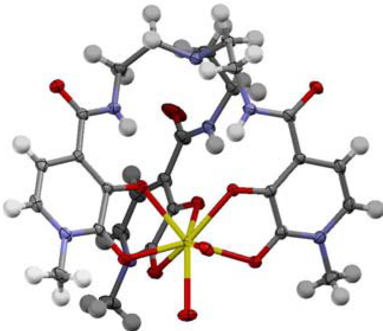
Figure 1. A view of the asymmetric unit for the [\text{Yb}(\text{Tren-Me-3,2-HOPO})(\text{H}_2\text{O})_2]\cdot 2\text{H}_2\text{O} complex. Non-coordinated solvent water molecules omitted for clarity and thermal ellipsoids are drawn at the 50 % probability level.
