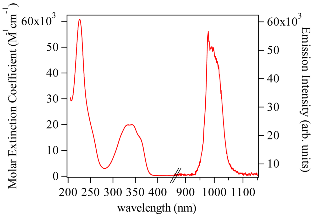
Figure 3. Electronic absorption spectrum in 0.1 M TRIS buffer at pH 7.4 (left) and steady state Near Infra-Red (NIR) emission spectrum in D 2 O (right) ( \lambda_{\text{ex}} = 345 nm, 10 nm bandpass) for the [Yb(Tren-Me-3,2-HOPO)(H 2 O) 2 ] complex.
