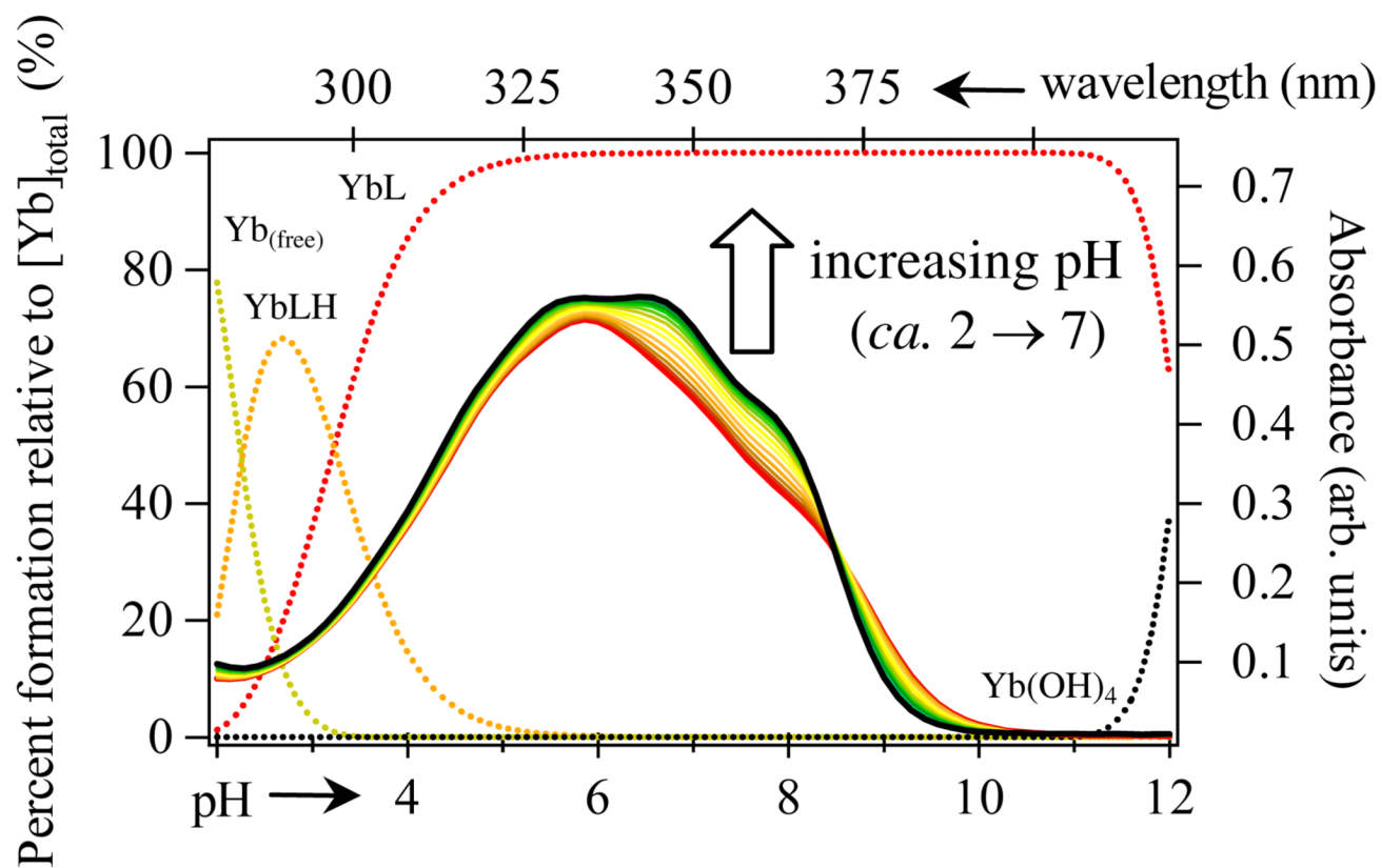
Figure 2. Speciation diagram of ca. 25 \mu\text{M} [\text{Yb}(\text{Tren-Me-3,2-HOPO})(\text{H}_2\text{O})_2] complex in aqueous solution (left, bottom axes) and overlaid changes in UV-Visible spectra (right, top axes) upon change in pH. red = free ligand spectrum ( ca. pH \sim 2), black = fully formed complex (above ca. pH 5.5 – 6).
