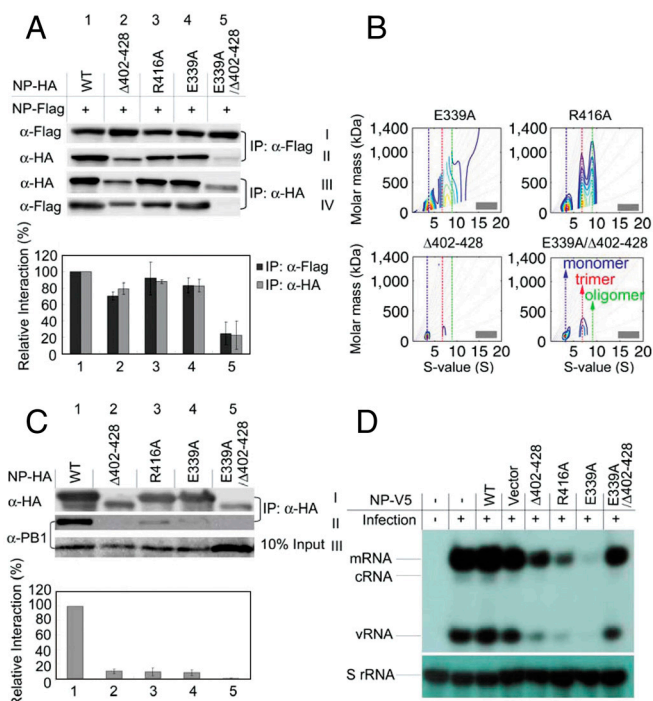
Fig. 2. IP assays of protein–protein interactions in cells. (A) Interaction of NP-FLAG with NP-HA or mutant-HA. 2 \times 10^6 HEK293T cells were cotransfected with 8 \mu g of each plasmid. IP analysis was performed 30 h post transfection using total cell extract by anti-FLAG and anti-HA agarose, and visualized by anti-FLAG and anti-HA antibodies. Black bar: row II/row I; gray bar: row IV/row III/row I. (B) AUC analyses to examine the ability of the NP mutants to mix with WT NP. The complete titration results at 6 different ratios are shown in Fig. S2; only the results of 1:1 ratio are shown here. Note that different y scales are used in the plots here and in Fig. S2 to show the best comparisons. (C) Pull-down assays for the interaction of NP proteins and PB1. The 2 \times 10^6 HEK293T cells were transfected with 8 \mu g of each plasmid separately (pCneo-NP-HA or pCneo-mutant-HA) for 24 h, then infected with the WSN virus (MOI = 0.2) for 12 h. IP analysis was performed using total cell extract by anti-HA agarose, and detected by anti-HA and anti-PB1 antibodies. The bar plots represent NP–PB1 interactions: row II/row III. The bar plots are means and SD from three independent experiments. (D) The transcription–replication activity is reduced by NP mutant proteins. MDCK cells were infected with the WSN virus at MOI of 2. RNA was isolated from cells 6 h after infection and analyzed by primer extension assays.
