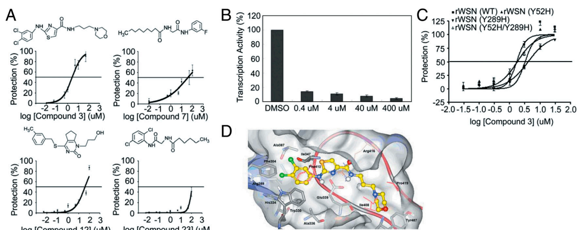
Fig. 5. Inhibition effects of small molecule inhibitors. (A) Structures and inhibitory effects of the compounds. The MDCK cells were incubated with compounds (0–100 μM), then inoculated with medium alone or the WSN virus (MOI = 0.001) for 48 h at 35 °C. The number of metabolically viable cells was determined. (B) In vitro transcription assay of compounds. The WSN viruses were incubated with compound 3 (0–400 μM) for 1 h at 25 °C. (C) The antiviral dose response curves of compound 3. The MDCK cells were incubated with the compound (0–100 μM), then inoculated with medium alone, the rWSN virus, nucleozin-resistant rWSN virus (Y289H mutation at NP), compound 3061-resistant rWSN virus (Y52H mutation at NP), or Y52H/Y289H double mutation rWSN virus (MOI = 0.001) at 35 °C. After 48 h, the number of metabolically viable cells was determined. (D) The modeled structure of the NP-compound 3 complex. The ribbon illustrates the NP tail-loop and the amino acids mentioned in the text are colored in pink. The compound 3 is shown in stick-and-ball with the carbon atoms colored in yellow. The NP residues interacting with compound 3 are showed in sticks.
