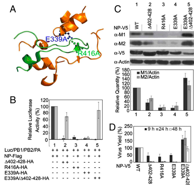
Fig. 1. Inhibition effect of NP mutants for the RDRP activity and viral replication. (A) Interactions involving the tail-loop (green) and its binding pocket (gold), from Protein Data Bank (PDB) 2IQH with PyMOL. (B) Luciferase-based reporter assays for reconstitution experiments, with 1 \mu g of each plasmid pPOLI-Luc-RT, pCneo-PB1, -PB2, -PA, and pCneo-NP-FLAG or -NP mutant-HA. The experiments were performed with and without pCneo-NP-FLAG. (C) The inhibition effects of NP mutant proteins on viral replication. 5 \times 10^5 MDCK cells (WT and mutant stable cell lines) were seeded per well and incubated for 24 h at 37 °C. Then cells were infected with the WSN virus at a multiplicity of infection (MOI) of 0.2. Western blot was performed at 9 h post infection using total cell extract. (D) MDCK cells (WT and mutant stable cell lines) were infected with the WSN virus at MOI of 0.2 as described in (C). The viral titers of the cell culture supernatant for viral replication were determined by plaque assays. The relative virus yields observed 9, 24, and 48 h postinfection are shown. The bar plots are means and SD from three independent experiments.
