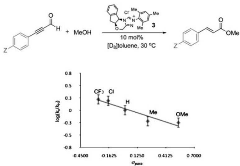
Figure 4. Linear free-energy relationship (Hammett study) for NHC-catalyzed redox reaction with para -substituted ynals: \rho = -0.69 ( Z = \text{CF}_3, \text{Cl}, \text{H}, \text{Me}, \text{or OMe} as indicated in the plot). \gamma = -0.6901 x + 0.0326 , R^2 = 0.903 .
