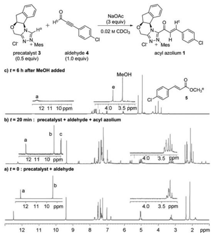
Figure 1. 1 H NMR investigation of \alpha,\beta -unsaturated acyl azolium 1 generated from 3 and 4 , and its methanolysis to 5 (the labeled H atoms correlate to the indicated signals in the spectra).
