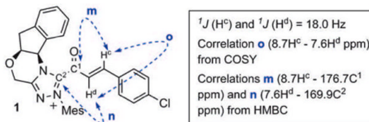
Figure 3. Key NMR correlation assignments of acyl azolium 1 .
