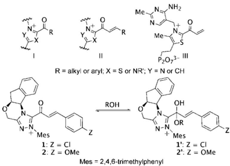
Scheme 1. Various acyl azoliums and the hemiacetals.
