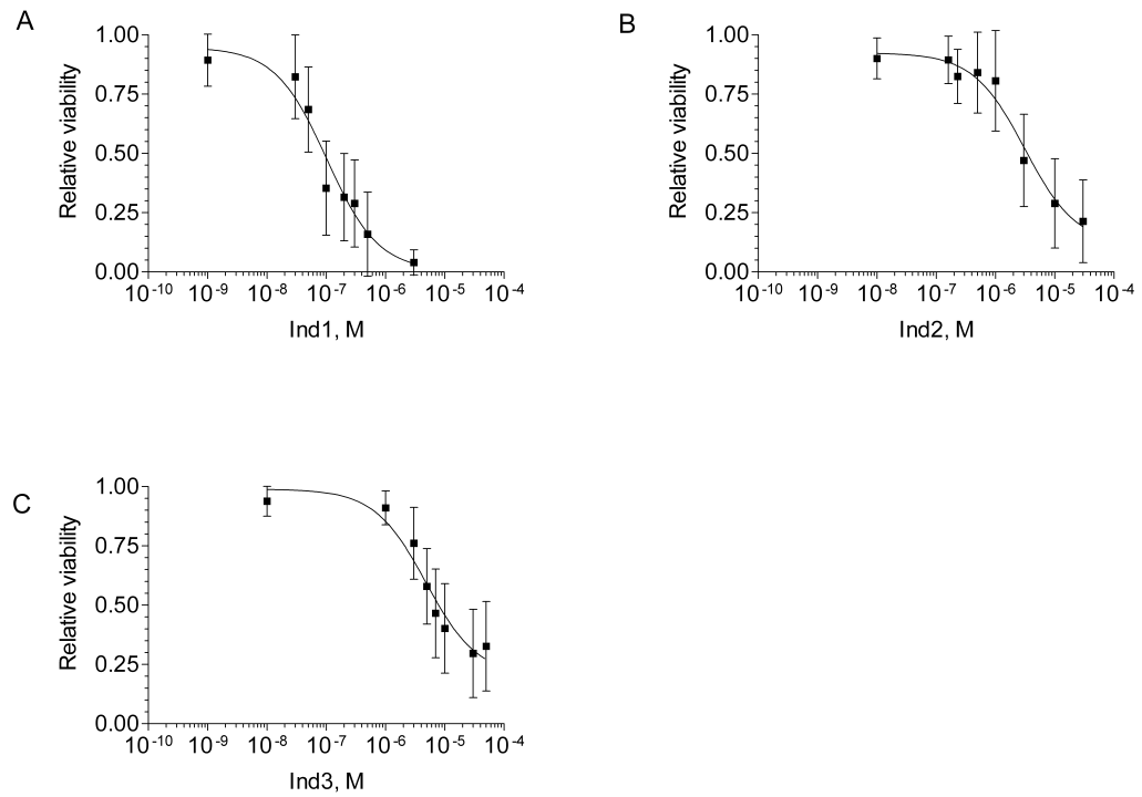
Figure 1. Concentration–response curve for (A) Ind1, (B) Ind2, and (C) Ind3. Data points represent the overall population mean (n=142) for growth inhibition relative to untreated controls at each concentration. Vertical bars represent the standard deviation for growth inhibition across the population.
