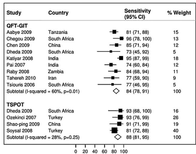
Figure 5. Sensitivity of QuantiFERON-TB Gold In-Tube and T-SPOT.TB among human immunodeficiency virus (HIV)-uninfected persons with confirmed active tuberculosis in low- and middle-income countries. The forest plots show the sensitivity estimates obtained from individual studies and pooled estimates derived from random effects (DerSimonian-Laird) modeling.
