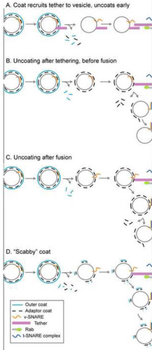
Figure 2. Models of vesicle uncoating
