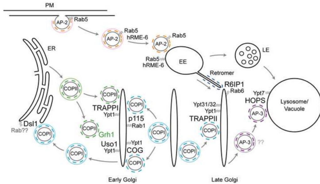
Figure 1. Overview of known coat-tether-Rab interactions
