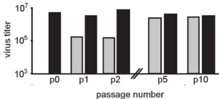
Figure 2. Serial passage in the presence of moderate concentrations of RNA mutagens selects for mutagen resistant populations. In this figure, Chikungunya virus was passaged in HeLa cells in the presence of 50 μM ribavirin (grey bars). Control passages were performed in absence of ribavirin (black bars). After each passage, virus progeny was quantified by classic plaque assay on BHK cells. The mutagenic effect is evident during the first passages (p1 and p2 compared to p0 starting population) where the treated virus titers drop by 2 log. Gradually, titers return to normal (untreated) levels. No significant differences are observed in passage 5 mutagen treated populations compared to untreated, suggesting that resistant variants have been selected. Indeed, consensus sequencing of the population identified unique mutations in the virus population undergoing ribavirin treatment.
