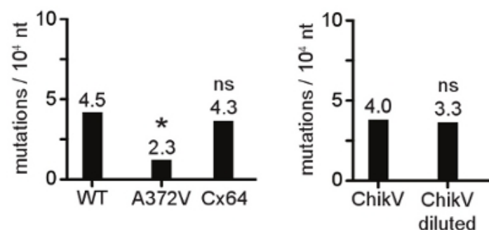
Figure 6. Graphic representation of mutation frequencies of virus populations. For easier interpretation, the numerical data obtained from sequence and statistical analyses can be represented as either a chart, or histogram (shown here). A372V virus generates fewer mutations than wild type and presents a significantly lower mutation frequency (*, p<0.01). The Cx64 variant, that replicates to titers 1000-fold lower than wild type, presents the same mutation frequency (ns, not significant) indicating that replication speed and fidelity are not necessarily linked. The same Chikungunya virus (CHIKV) population gives similar mutation frequencies whether the virus stock, or a 10 5 -fold dilution, is used for RNA extraction.
