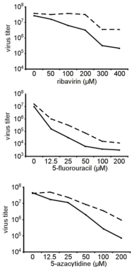
Figure 3. Confirmation of broad resistance to RNA mutagens of different structure. Shown here, the high fidelity A372V variant of Coxsackie virus B3 that was initially isolated in the screen described in Section 3 was generated from an infectious clone and tested for its relative sensitivity to different concentrations of different RNA mutagens (ribavirin, 5-fluorouracil, 5-azacytidine). HeLa cells were treated with indicated concentrations of ribavirin and infected with wild type Coxsackie virus B3 at a MOI of 0.01. 48 hours post infection, the progeny virus was harvested and titers were determined by TCID 50 . Shown here are the titers of wild type (solid lines) and A372V variant (dashed lines) as a function of mutagen concentration. A372V consistently titers higher than wild type under all conditions tested.
