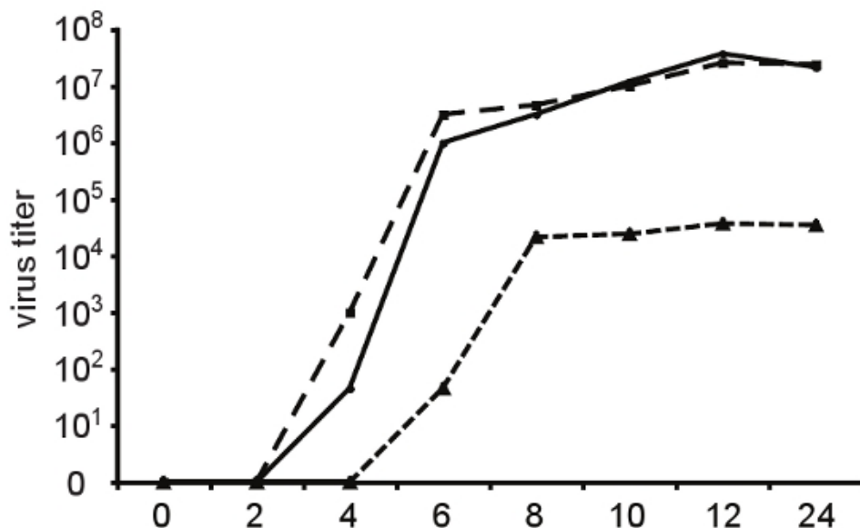
Figure 3. Confirmation of broad resistance to RNA mutagens of different structure. Shown here, the high fidelity A372V variant of Coxsackie virus B3 that was initially isolated in the screen described in Section 3 was generated from an infectious clone and tested for its relative sensitivity to different concentrations of different RNA mutagens (ribavirin, 5-fluorouracil, 5-azacytidine). HeLa cells were treated with indicated concentrations of ribavirin and infected with wild type Coxsackie virus B3 at a MOI of 0.01. 48 hours post infection, the progeny virus was harvested and titers were determined by TCID 50 . Shown here are the titers of wild type (solid lines) and A372V variant (dashed lines) as a function of mutagen concentration. A372V consistently titers higher than wild type under all conditions tested.
