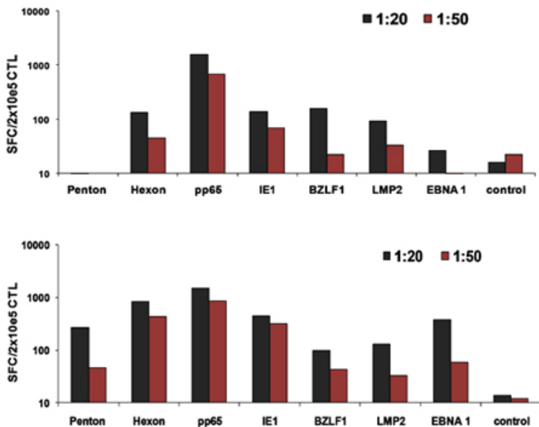
Figure 3. Optimal DC:T cell ratios for CTL activation. DCs from 2 donors were nucleofected with all three optimized plasmids and then used to stimulate autologous PBMCs at 1:20 or 1:50 DC:PBMC ratio. The frequency of reactivated T cells was assessed on day 10 by IFN \gamma ELISpot.
