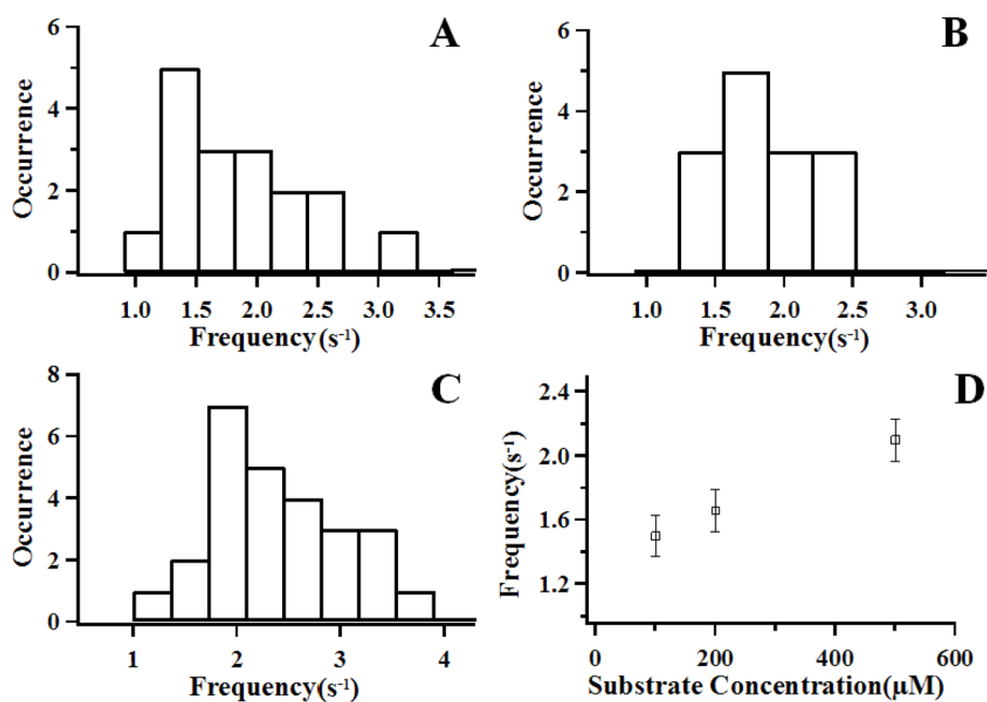
Figure 3. The distributions of coherence frequency of the conformational change fluctuations under enzymatic reactions with various substrate concentrations. (A) 100 \mu M ATP + 100 \mu M HP; (B) 200 \mu M ATP + 200 \mu M HP; (C) 500 \mu M ATP + 500 \mu M HP; (D) Statistical results of coherence frequency distribution in enzymatic reaction under various substrate concentrations.
