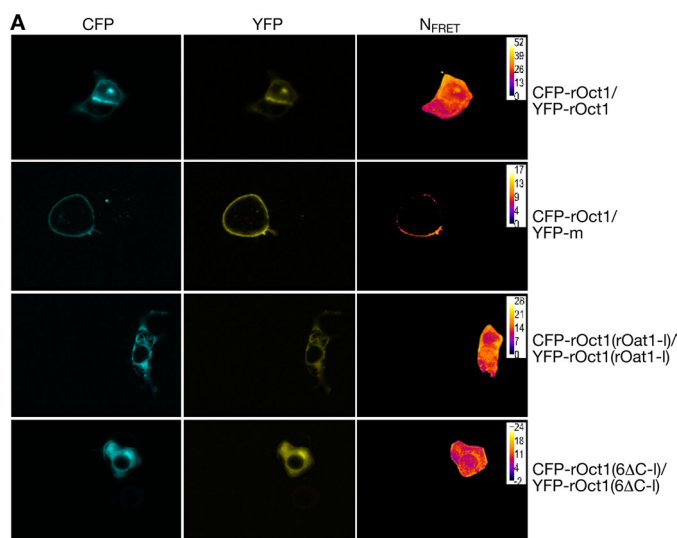
FIGURE 7. Oligomerization of rOct1, rOct1(rOat1-l), and rOct1(6ΔC-l) as demonstrated by FRET microscopy in intact cells. A, FRET images. HEK 293 cells were transiently transfected with cDNAs encoding CFP- and YFP-tagged rOct1, CFP-tagged rOct1, and membrane-associated YFP ( m -YFP), CFP- and YFP-tagged rOct1(rOat1-l), and CFP- and YFP-tagged rOct1(6ΔC-l). Two days after transfection, epifluorescence microscopy was performed. The first and second columns show images obtained with CFP and YFP filter sets; the third column displays a corrected and normalized FRET image ( N_{FRET} ) established with PIX-FRET. The color code is presented in the last column. In all images, background fluorescence was subtracted. The indicated images are representative of 4–8 experiments. B, normalized FRET efficiencies ( N_{FRET} values). Mean ± S.E. (error bars) values are indicated. The numbers of measured cells are given in parentheses. ***, p < 0.001 , difference from rOct1-w; ●●●, p < 0.001 . The data indicate that the large extracellular loop is pivotal for oligomerization.
