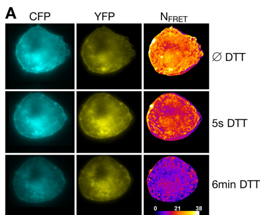
FIGURE 8. Oligomerization of rOct1 expressed in HEK293 cells is destroyed after incubation with DTT. A, FRET images. HEK 293 cells were transiently transfected with cDNAs encoding CFP- and YFP-tagged rOct1. Two days after transfection, epifluorescence microscopy was performed without DTT incubation, after incubation for 5 s with 10 mM DTT, and after incubation for 6 min with 10 mM DTT. The first and second column show images obtained with CFP and YFP filter sets, whereas the third column displays a corrected and normalized FRET image ( N_{FRET} ). Representative images with subtracted background fluorescence are shown. B, normalized FRET efficiencies ( N_{FRET} values). Mean ± S.E. (error bars) values are indicated. The numbers of measured cells are given in parentheses. *, p < 0.05 ; ***, p < 0.001 . The experiment suggests that reduction of disulfide bridges within the large extracellular loop rapidly alters the equilibrium between rOct1 monomers and oligomers in the plasma membrane.
