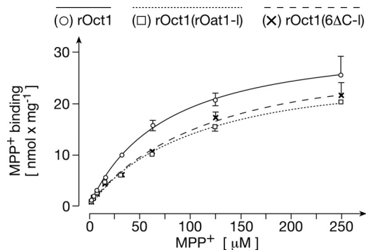
FIGURE 5. Comparison of MPP + binding to rOct1, rOct1(rOat1-1), and rOct1(6 \Delta C-1). Binding of [ 3 H]MPP + was measured to rOct1 (○, solid line), rOct1(rOat1-1) (□, dotted line), and rOct1(6 \Delta C-1) (×, dashed line). The transporters were synthesized by cell-free expression, solubilized with LMPG, purified in the presence of CHAPS, and precipitated by detergent removal via dialysis. Binding of 12 nM [ 3 H]MPP + was measured in the presence of the indicated total MPP + concentrations and in the presence of 5 mM nonradioactive MPP + . [ 3 H]MPP + binding replaced by 5 mM MPP + was calculated. Mean values \pm S.D. from four parallel measurements of three typical experiments are indicated. A one-site binding curve was fitted to the data. The K_D values of 119 \pm 23 \mu M (rOct1(6 \Delta C-1)), 113 \pm 32 \mu M (rOct1(Oat1-1)), and 77 \pm 8.6 \mu M (rOct1 wild type) were obtained. The difference between rOct1 wild type and rOct1(6 \Delta C-1) was significant in Student's t test ( p < 0.05).
