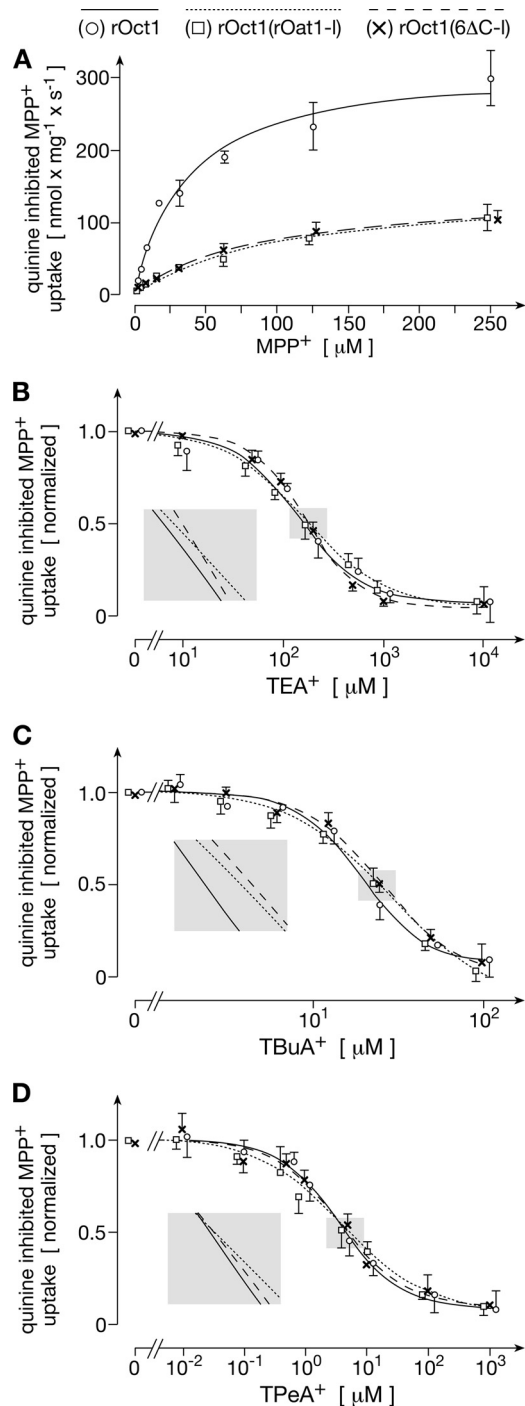
FIGURE 6. Comparison of MPP + uptake into proteoliposomes containing rOct1, rOct1(rOat1-l), and rOct1(6ΔC-l). His-tagged transporters were expressed in vitro and purified, and 60 μg of individual transporters were reconstituted into proteoliposomes containing 100 mM potassium cyclamate. After preincubation with valinomycin, proteoliposomes were incubated for 1 s with 12 nM [ 3 H]MPP + plus various concentrations of nonlabeled MPP + (A) TEA + (B), TBuA + (C), or TPpA + (D). The incubation buffer contained 90 mM Na + , 10 mM K + , and 100 mM cyclamate - . Measurements were performed in the absence and presence of 100 μM quinine, and quinine-inhibited uptake is indicated. Means ± S.D. (error bars) of three measurements from individual experiments are shown. The Michaelis-Menten equation was fitted to the data in A, whereas the Hill equation was fitted to the data in B–D. In the insets, fitted curves close to the calculated IC 50 values are enlarged.
