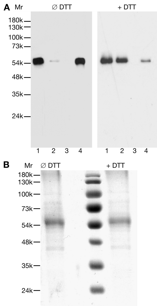
FIGURE 3. Homo-oligomerization of solubilized rOct1 in the presence of LMPG and CHAPS is prevented by reduction of intramolecular disulfide bridge(s). A , effect of DTT on coprecipitation of solubilized FLAG-tagged rOct1 wild type with solubilized His-tagged rOct1. The experimental protocol described in the legend to Fig. 2 was used, and the data are presented as in Fig. 2. Coprecipitation of solubilized proteins in the presence of LMPG plus CHAPS was performed without DTT and with 10 mM DTT in the solubilization buffer. B , exclusion of intermolecular disulfide bridges between rOct1 monomers. The mixtures of solubilized FLAG-tagged and His-tagged rOct1 wild type proteins used for coprecipitation in Fig. 3 A were separated by SDS-PAGE either in the presence or absence of DTT in the sample buffer and stained with Coomassie Brilliant Blue.
