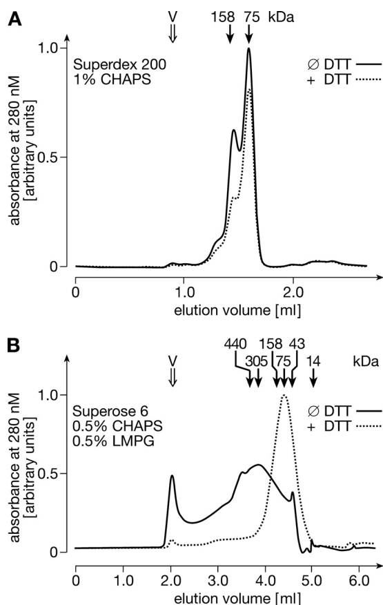
FIGURE 4. Gel filtration chromatography of solubilized rOct1 wild type in the presence of LMPG and CHAPS performed under non-reducing and reducing conditions. Cell-free expressed rOct1 protein was solubilized with 2% LMPG and concentrated to 4 mg/ml protein, and 40 \mu l were applied to a Superdex 200 column (A) or to a tandem of two coupled Superose 6 PC 3.2/30 columns (B). The columns were equilibrated and operated with 20 mM Tris/HCl, pH 8, containing 500 mM NaCl and either 1% CHAPS (A) or 0.5% LMPG plus 0.5% CHAPS using a flow rate of 50 \mu l/min (A) or 0.28 ml/min (B). In one series of experiments, 10 mM DTT was added to the sample buffer, and in another series of experiments, DTT was omitted. The indicated molecular weights were obtained by calibration of the columns with ferritin (440 kDa), aldolase (158 kDa), conalbumin (75 kDa), ovalbumin (43 kDa), and ribonuclease A (14 kDa). The data suggest that under non-reducing conditions, rOct1 wild type forms dimers in the presence of 1% CHAPS and tetramers in the presence of 0.5% CHAPS and 0.5% LMPG.
