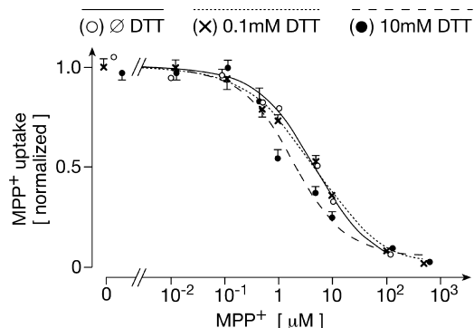
FIGURE 9. Incubation of rOct1 expressed in HEK293 cells with DTT alters transport kinetics. Cells were preincubated for 6 min with PBS containing 10 mM DTT, washed with PBS containing 0.1 mM DTT, and incubated for 10 min in the same buffer (●). Control cells were preincubated, washed, and incubated with PBS (○) or PBS containing 0.1 mM DTT (×). Substrate concentration dependence of MPP + uptake into HEK293 cells stably transfected with rOct1 was measured in the absence of DTT (○) or in the presence of 0.1 mM DTT (×, ●). Mean values ± S.D. (error bars) of 12–16 measurements from three or four experiments are presented. The uptake rates of the individual measurements are normalized. The Hill equation is fitted to the data.
