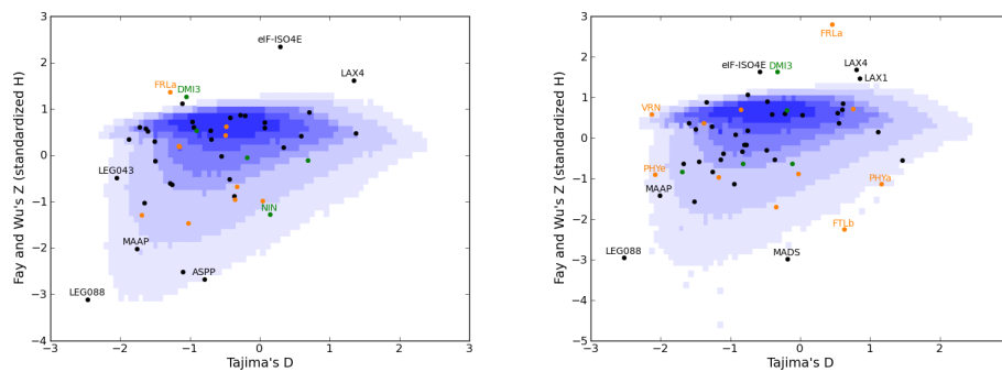
Figure 3 Tests of selective neutrality of polymorphism within each group. The joint distributions of ( D , Z ) tests statistics expected under neutrality in the Eastern group (group 1, panel 3a) and the Western group (group 2, panel 3b) are plotted using a blue shading for the probability density. Symbiotic genes are plotted as green dots and flowering genes as orange dots using each candidate gene abbreviation. Control loci are represented as black dots. The joint distribution for ( D , Z ) within each group was obtained through 10^5 coalescent simulations from models parametrized to fit patterns of polymorphisms in the set of controlled fragments (See Methods for further details). Note that in order to generate a unique graphical representation of the neutral joint distribution, simulations for each of the 53 loci were pooled and the resulting ( D , Z ) distribution was binned using 10^4 categories (rigorous p-values computed using null distributions tailored for each locus length and polymorphism are available in Additional file 7, Table S5).
