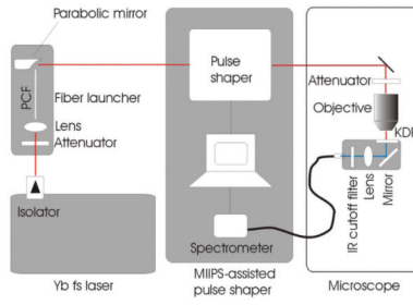
Fig. 1. (Color online) TL compression of fiber SC pulses in a high-NA focus.
