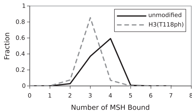
Figure 3. Distribution of the number of bound hMSH2-hMSH6 complexes needed to displace nucleosomes from the 601 positioning sequence. The solid line shows the result for unmodified nucleosomes, and the dashed line for the dyad modification H3(T118ph).
