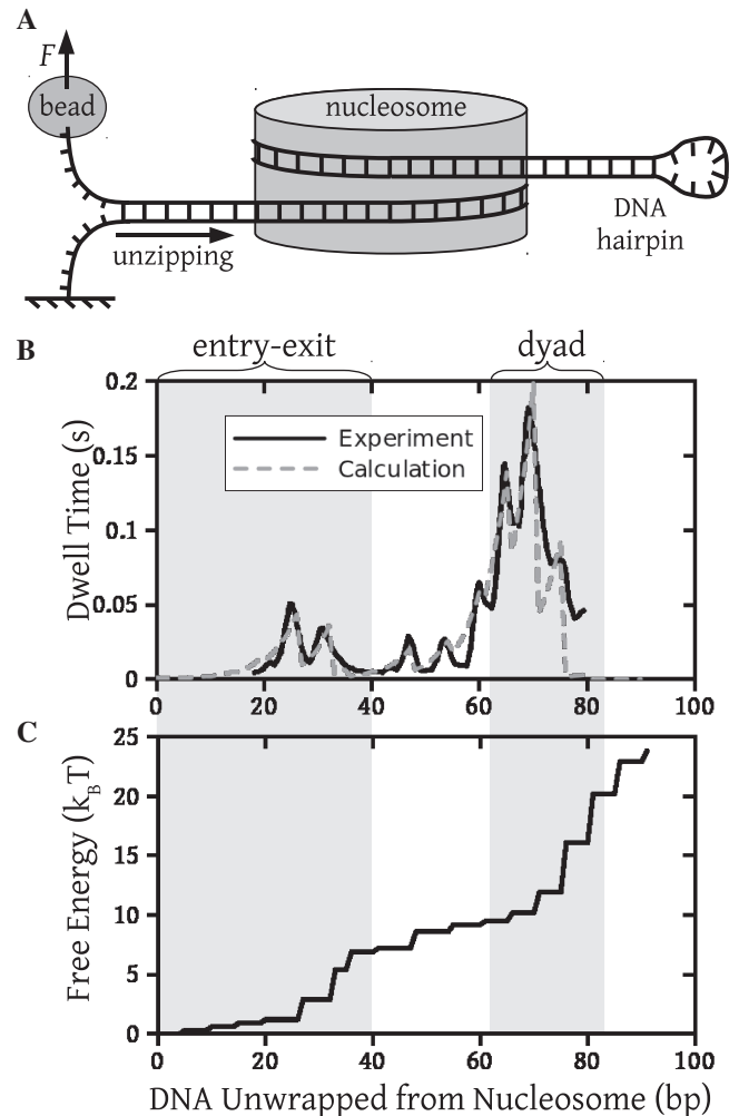
Figure 1. A free energy landscape consistent with measurements of mechanical unzipping of nucleosomes. (A) Experimental setup for unzipping experiments. One strand of the DNA is attached to a surface, and a constant force F of 28 pN is applied to the other end via a bead in an optical trap, slowly pulling apart the DNA base pairing. As this unzipping of the base pairing moves through the nucleosome, the DNA must also be unwrapped from the nucleosome. (B) Dwell time as a function of the number of DNA base pairs (bp) unwrapped from the nucleosome. The solid line is determined from mechanical unzipping experiments, while the dashed line is calculated from (C) the free energy landscape for DNA unwrapping from a nucleosome on the 601 positioning sequence. Significant pauses when 20–30 bp are unwrapped (within the entry–exit region) and when 60–80 bp are unwrapped (within the dyad region) correspond to areas where the free energy landscape changes rapidly.
