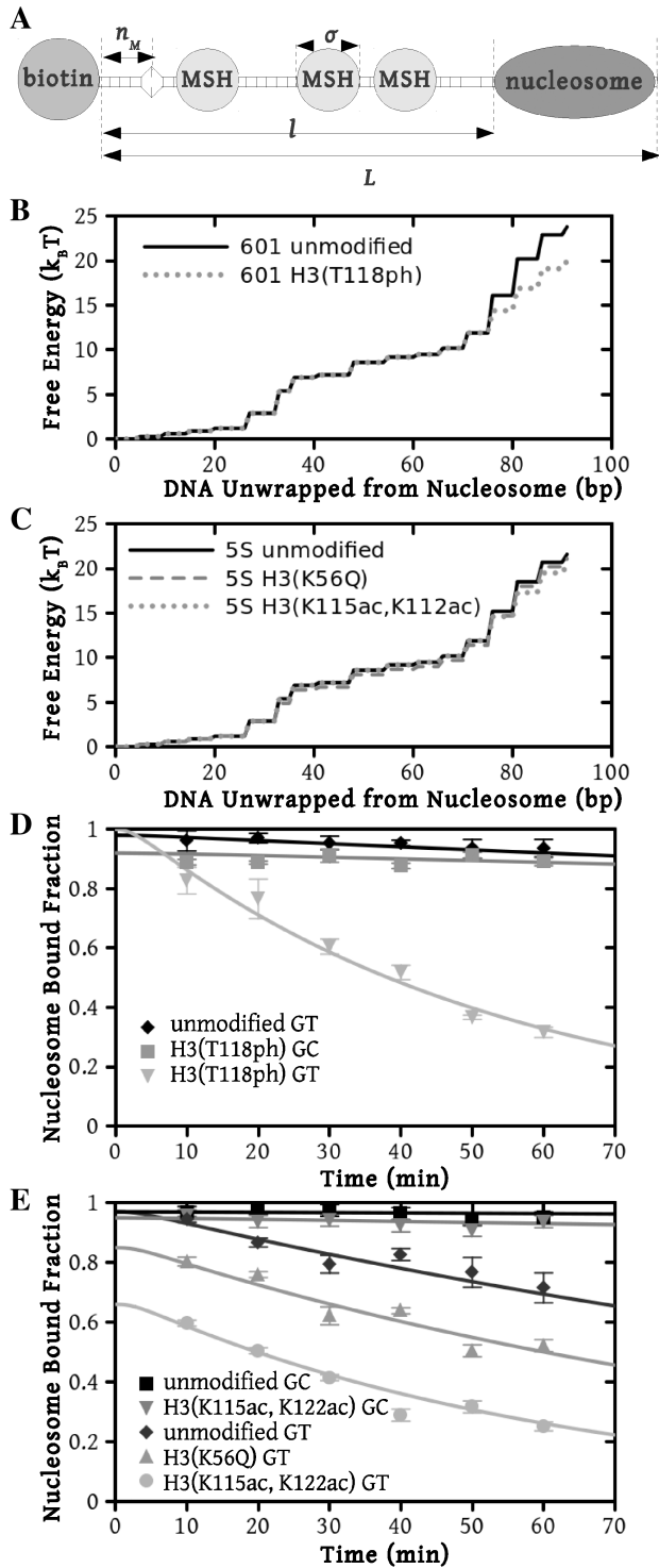
Figure 2. Model predictions compared with experimental measurements for nucleosome displacement by hMSH2-hMSH6. (A) Graphical depiction of the experimental system [10]. Streptavidin bound to the biotinylated left end of the DNA prevents hMSH2-hMSH6 (MSH) from sliding off this end, while a nucleosome inhibits hMSH2-hMSH6 from sliding off the right end of the DNA. There is a mismatch located n_M = 21 bp from the biotin bead, at which hMSH2-hMSH6 may bind. The total length of the DNA segment is L . The hMSH2-hMSH6 is confined to length l , the DNA between the biotin bead and the nucleosome. The footprint of one hMSH2-hMSH6 molecule is \sigma = 25 bp. Free energy landscapes for unwrapping nucleosomes on (B) the 601 positioning sequence and (C) the 5S positioning
