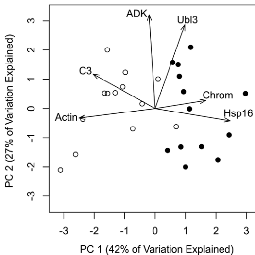
Figure 4. Principal components analysis of stress response gene expression in Porites astreoides . Black circles represent heat-light treated samples ( n = 13 ), white circles represent control samples ( n = 13 ). Vectors indicate loadings for each gene. The two major loadings on PC1 are Hsp16 (0.55) and actin (-0.56). Abbreviations are as follows: C3 = complement component C3; ADK = adenosine kinase; Ubl3 = Ubiquitin-like protein 3; Chrom = GFP-like chromoprotein. doi:10.1371/journal.pone.0026914.g004
