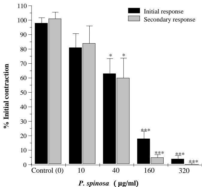
Fig. 4. Inhibitory effect of Pycnocykla spinosa root extract on biphasic contractions of rat ileum induced by electrical field stimulation. Results are given as mean and vertical bars indicate SEM (n=6). Stars show statistically significant differences between extract and the initial controls. * P < 0.05 , *** P < 0.001 (Student's t-test).
