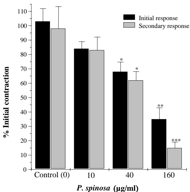
Fig. 5. Inhibitory effects of Pycnocykla spinosa aerial extract on biphasic contractions of rat ileum induced by electrical field stimulation. Results are given as mean and vertical bars indicate SEM (n=6). Stars show statistically significant differences between extract and the initial controls. * P < 0.05 , ** P < 0.01 , *** P < 0.001 (Student's t-test).
